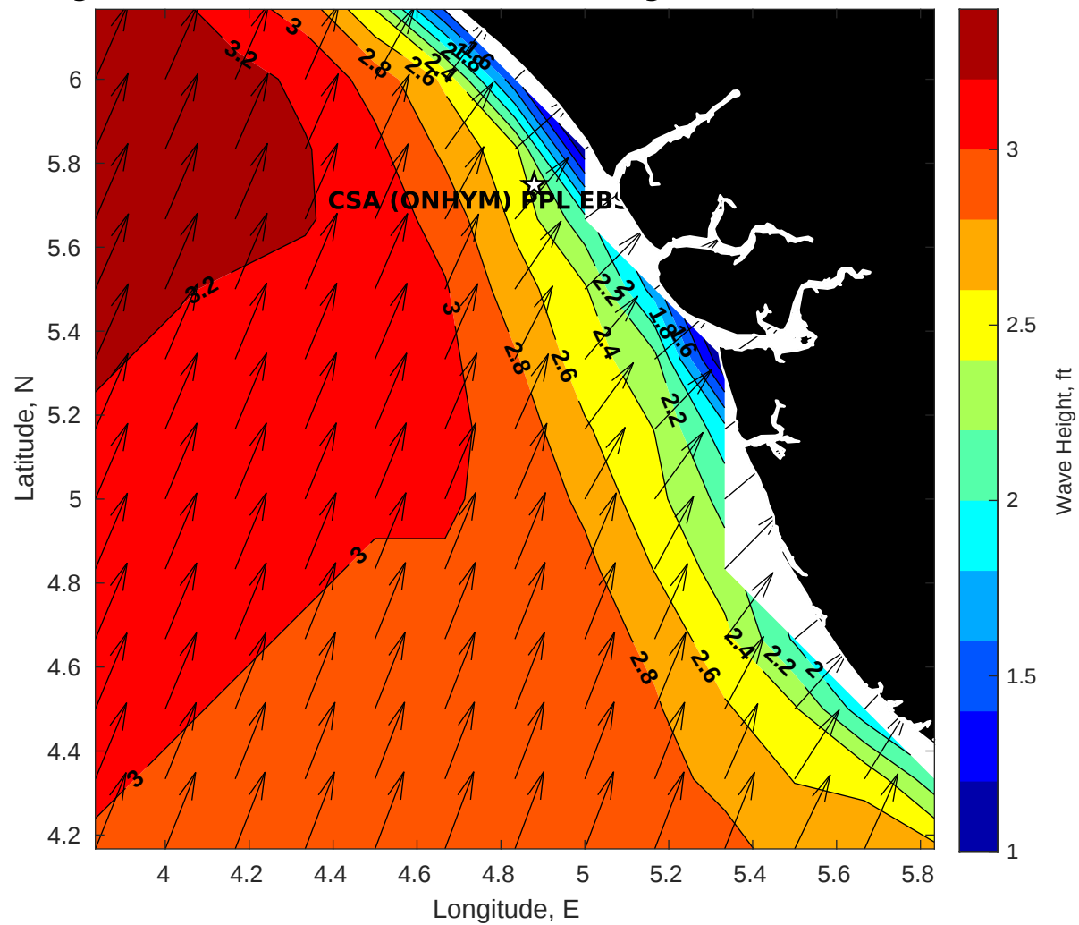
Wave Height (ft) for CSA (ONHYM) PPL EBS - Nigeria at 02-Mar-2025 09:00:00
