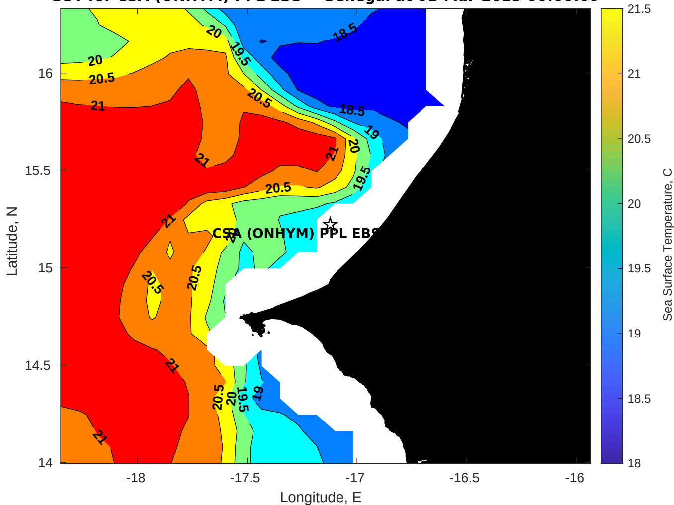
SST for CSA (ONHYM) PPL EBS - Senegal at 01-Mar-2025 00:00:00
