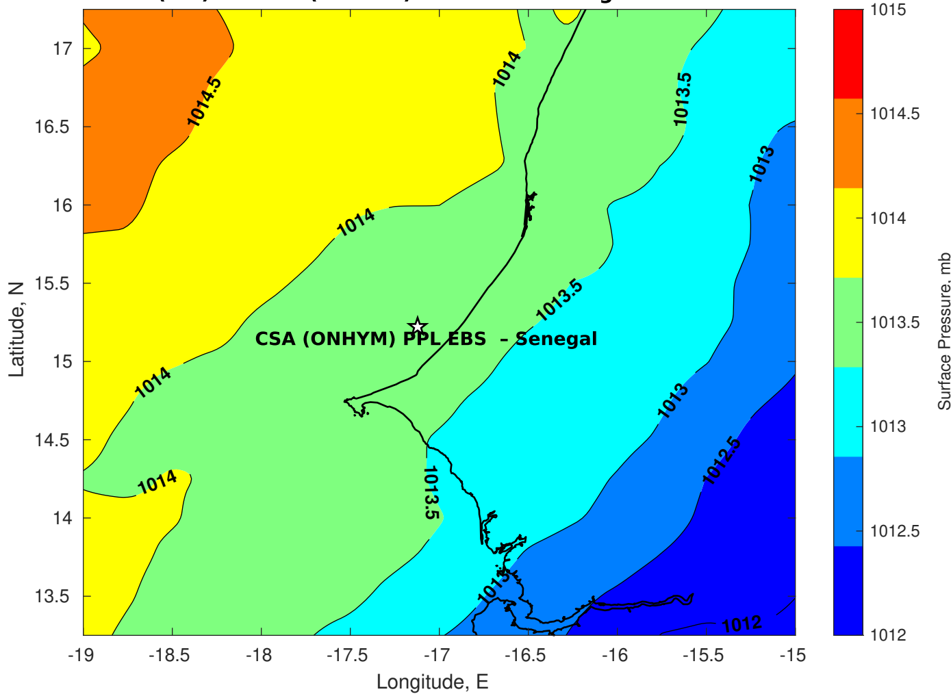
Surface Pressure (mb) for CSA (ONHYM) PPL EBS - Senegal at 04-Mar-2025 00:00:00
