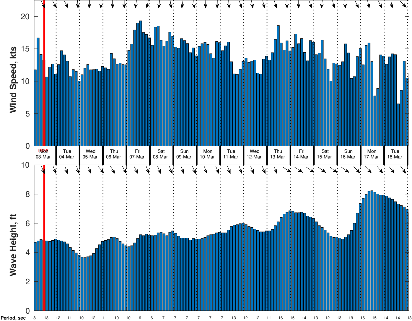
Wind & Wave Forecast for CSA (ONHYM) PPL EBS - Senegal from 02-Mar-2025 01:00:00 to 18-Mar-2025 01:00:00
