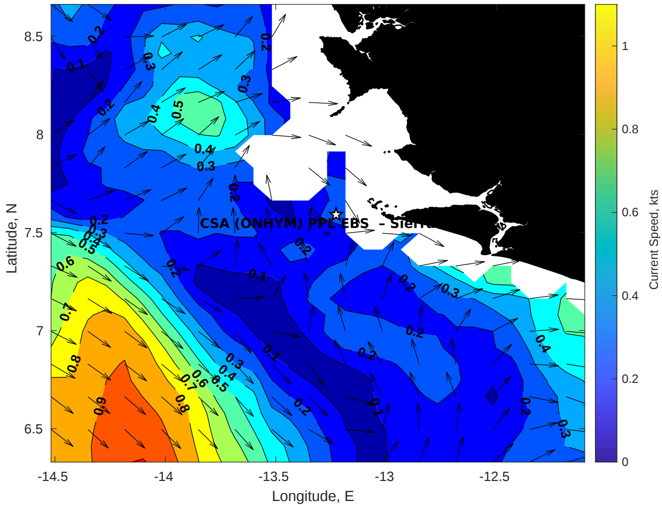
Surface Currents for CSA (ONHYM) PPL EBS - Sierra Leone at 01-Mar-2025 00:00:00
