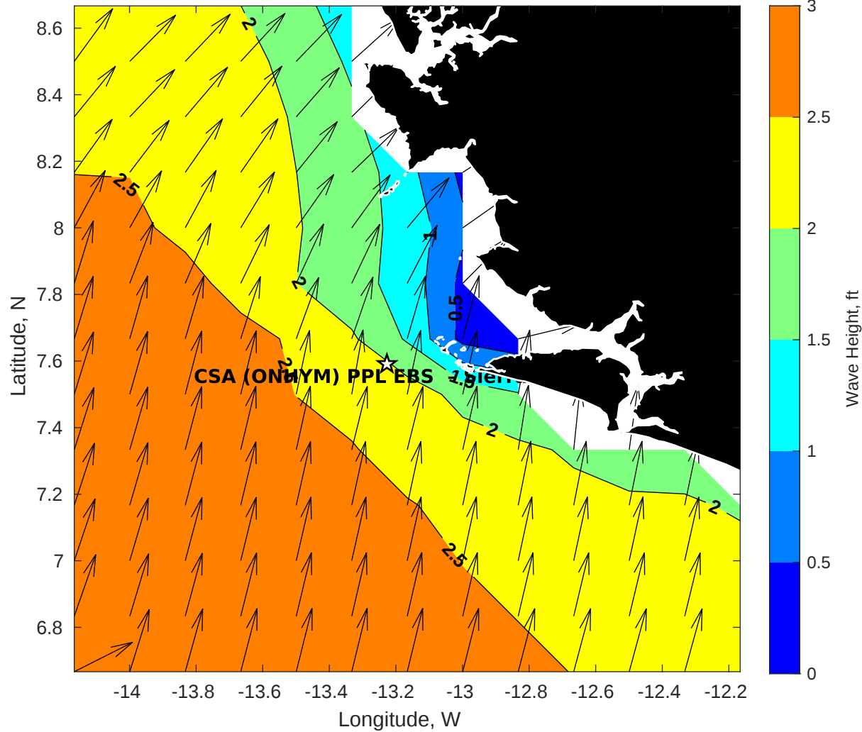
Wave Height (ft) for CSA (ONHYM) PPL EBS - Sierra Leone at 02-Mar-2025 09:00:00
