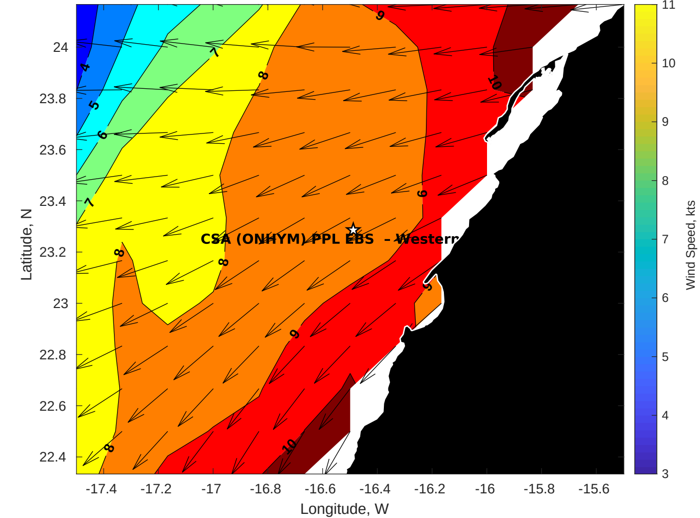
Winds (kts) for CSA (ONHYM) PPL EBS - Western Sahara at 02-Mar-2025 09:00:00
