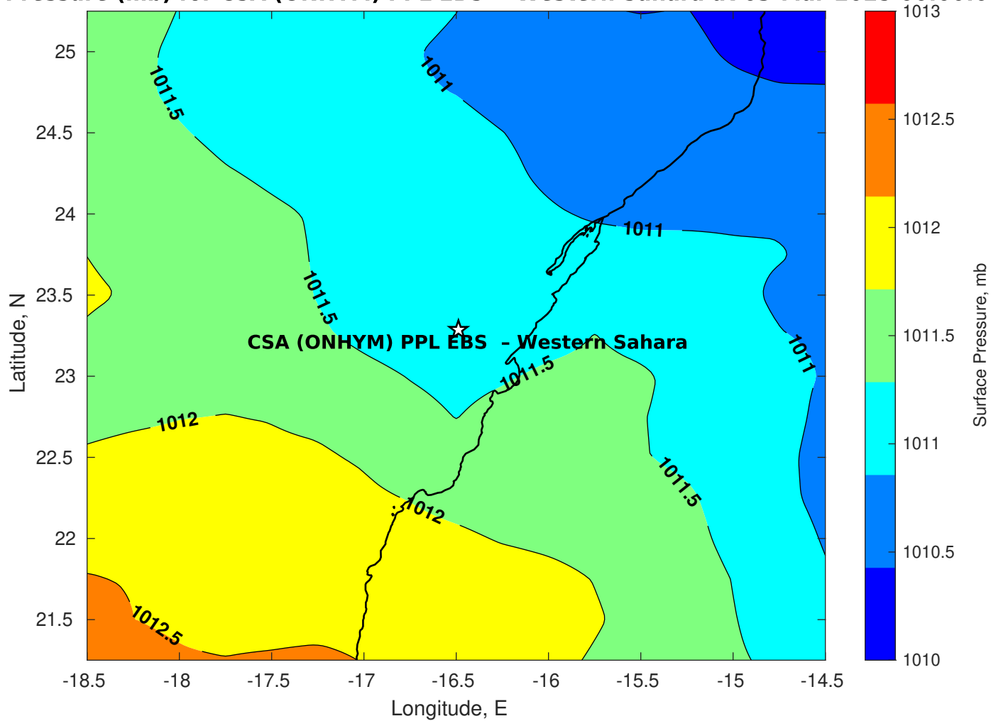
Surface Pressure (mb) for CSA (ONHYM) PPL EBS - Western Sahara at 03-Mar-2025 00:00:00
