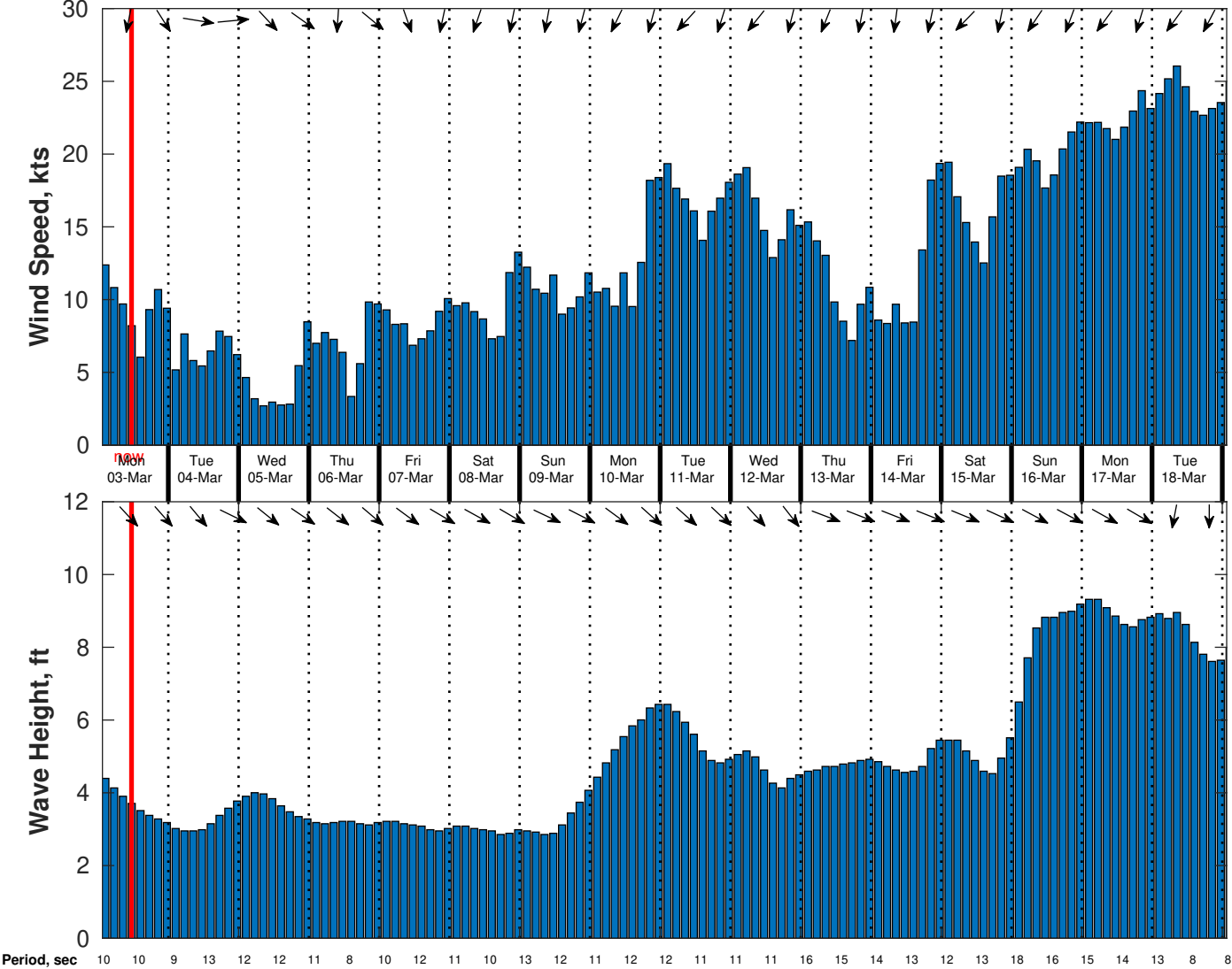
Wind & Wave Forecast for CSA (ONHYM) PPL EBS - Western Sahara from 02-Mar-2025 01:00:00 to 18-Mar-2025 01:00:00
