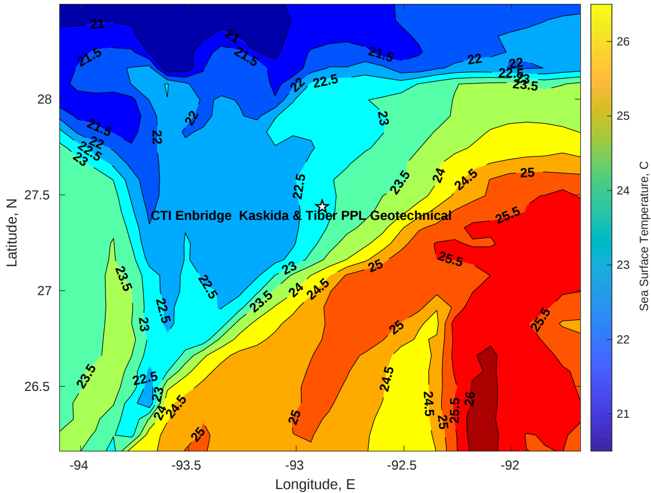
SST for CTI Enbridge Kaskida & Tiber PPL Geotechnical at 01-Mar-2025 00:00:00
