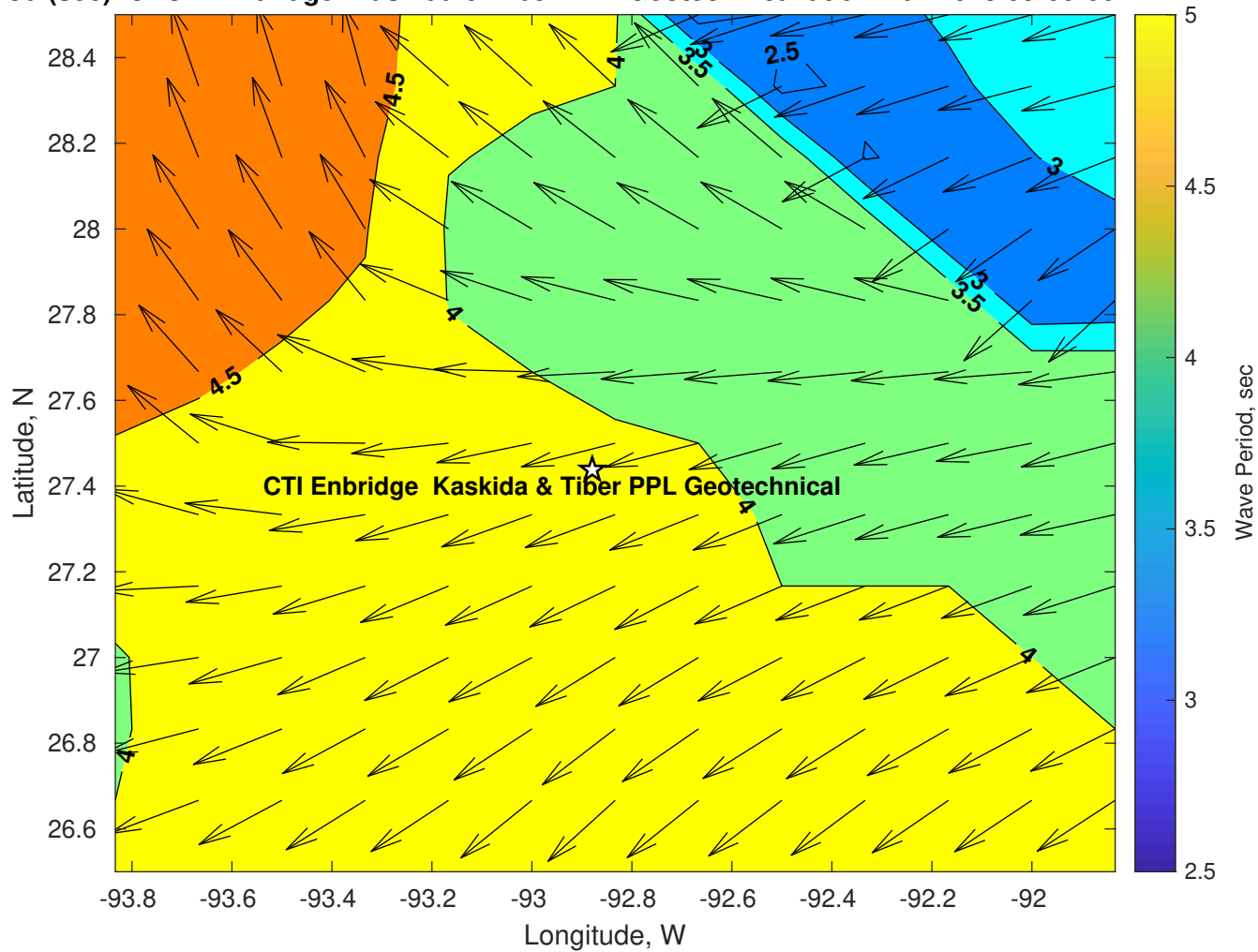
Wave Period (sec) for CTI Enbridge Kaskida & Tiber PPL Geotechnical at 02-Mar-2025 09:00:00
