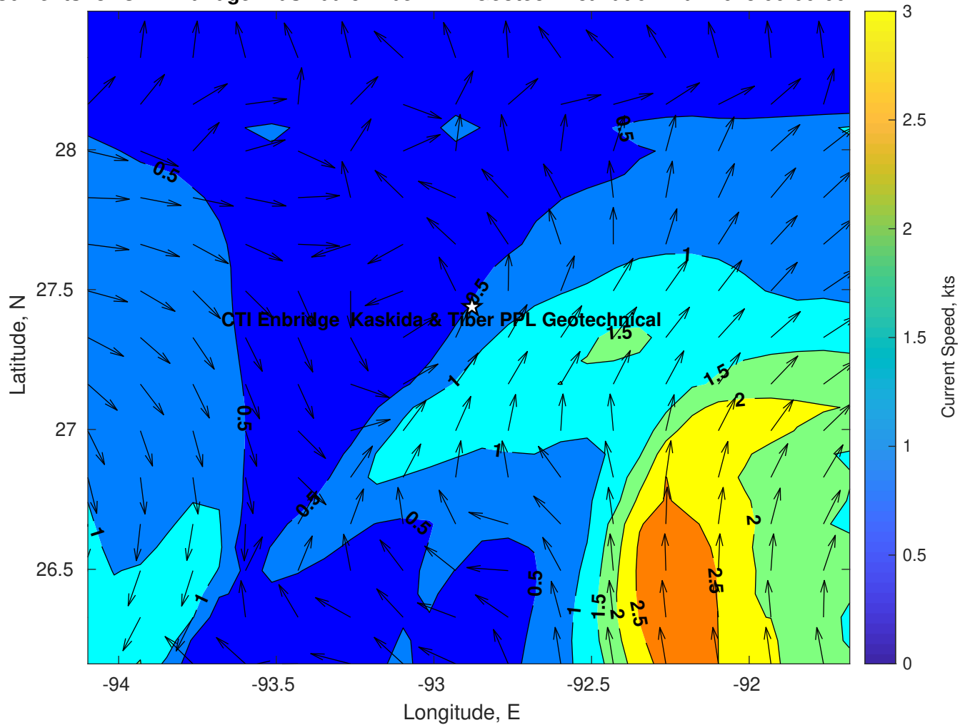
Surface Currents for CTI Enbridge Kaskida & Tiber PPL Geotechnical at 01-Mar-2025 00:00:00
