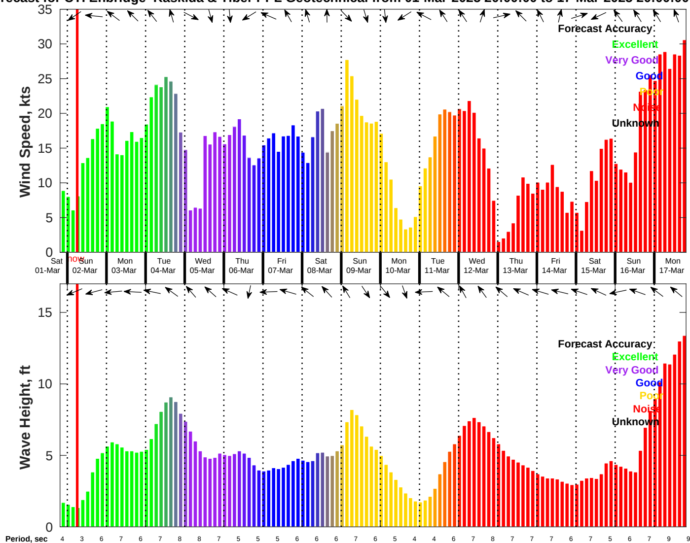
Wind & Wave Forecast for CTI Enbridge Kaskida & Tiber PPL Geotechnical from 01-Mar-2025 20:00:00 to 17-Mar-2025 20:00:00
