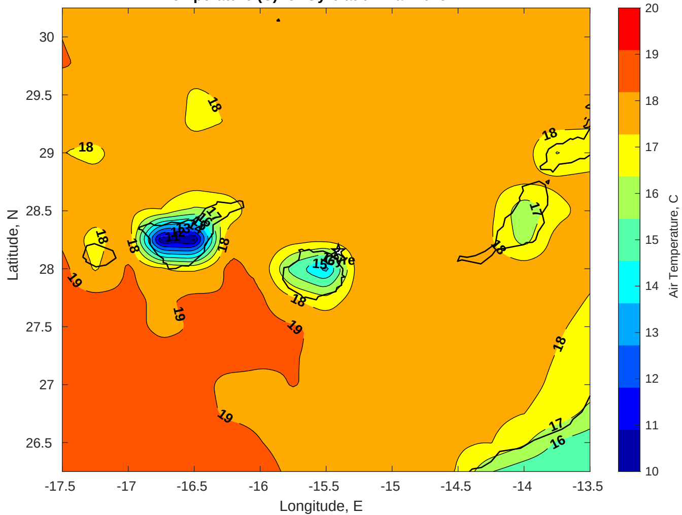
Air Temperature (C) for Gyre at 02-Mar-2025
