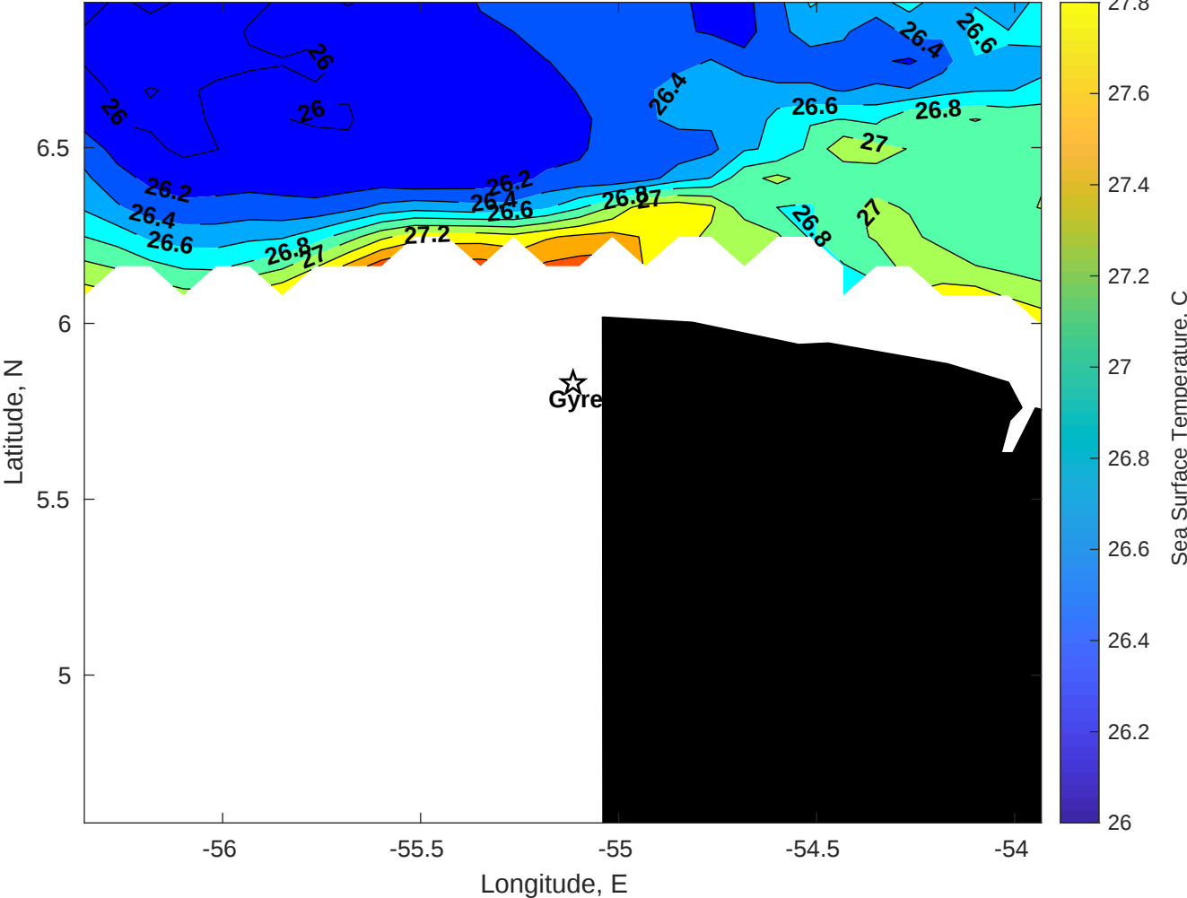
SST for Gyre at 01-Mar-2025 00:00:00
