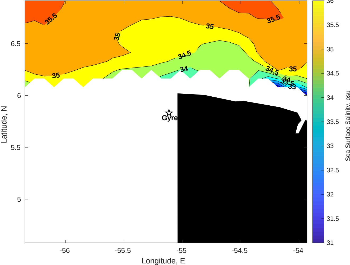
Surface Salinity for Gyre at 01-Mar-2025 00:00:00
