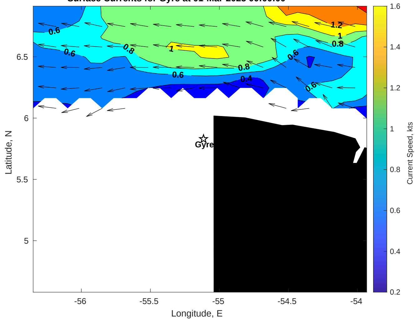
Surface Currents for Gyre at 01-Mar-2025 00:00:00
