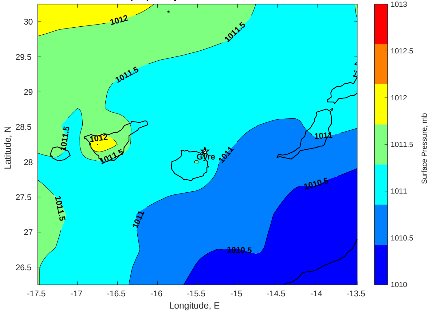
Surface Pressure (mb) for Gyre at 03-Mar-2025 00:00:00
