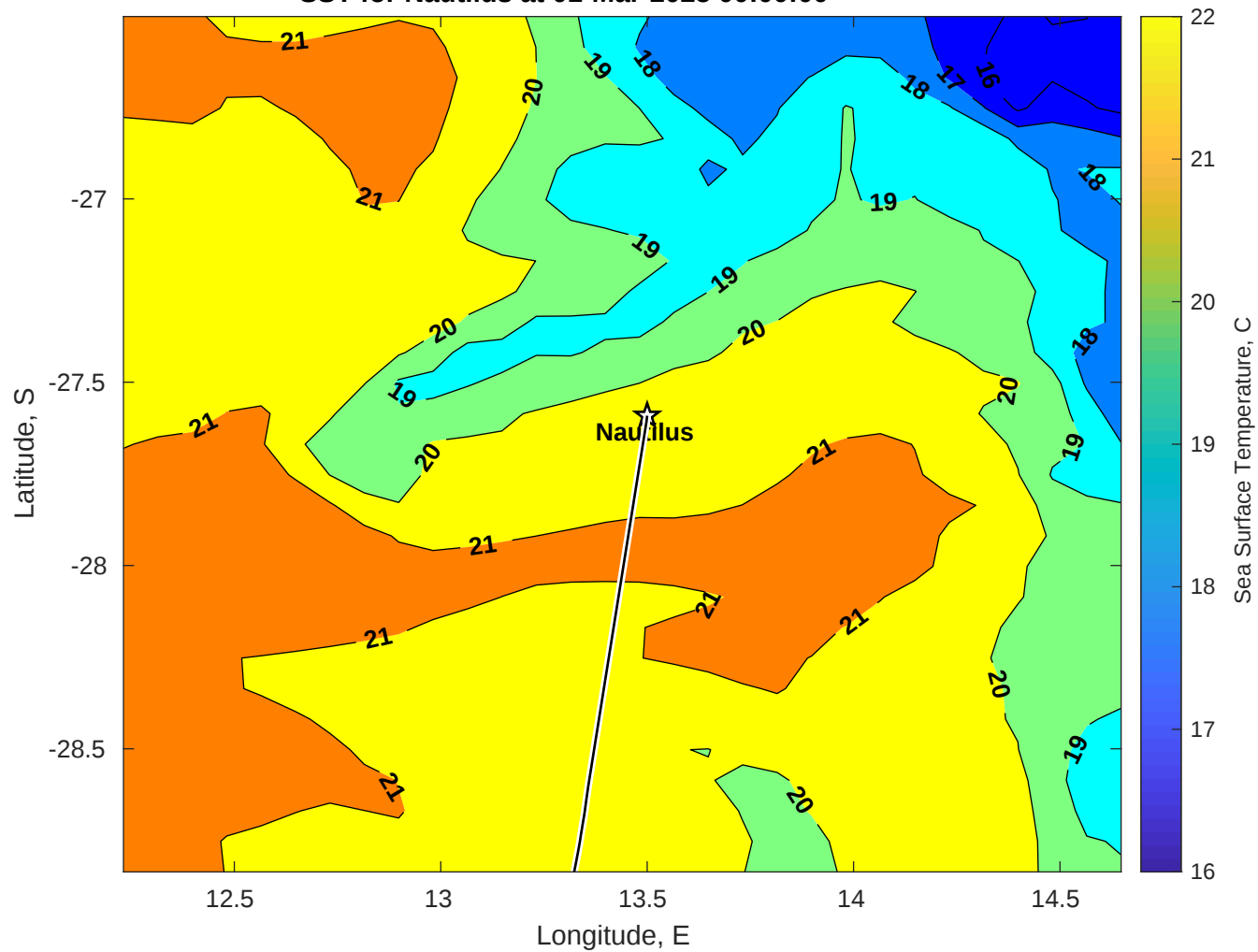
SST for Nautilus at 01-Mar-2025 00:00:00
