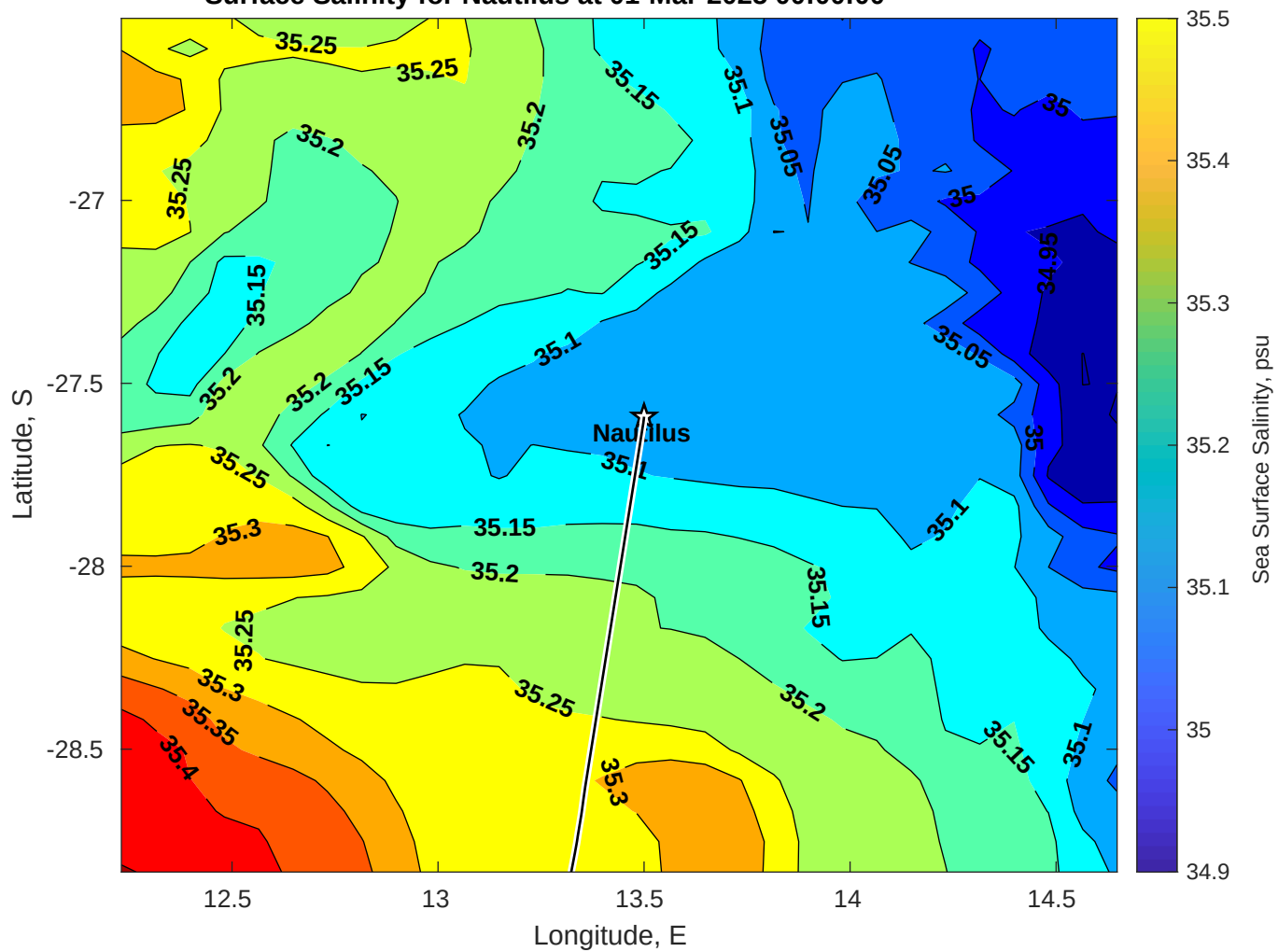
Surface Salinity for Nautilus at 01-Mar-2025 00:00:00
