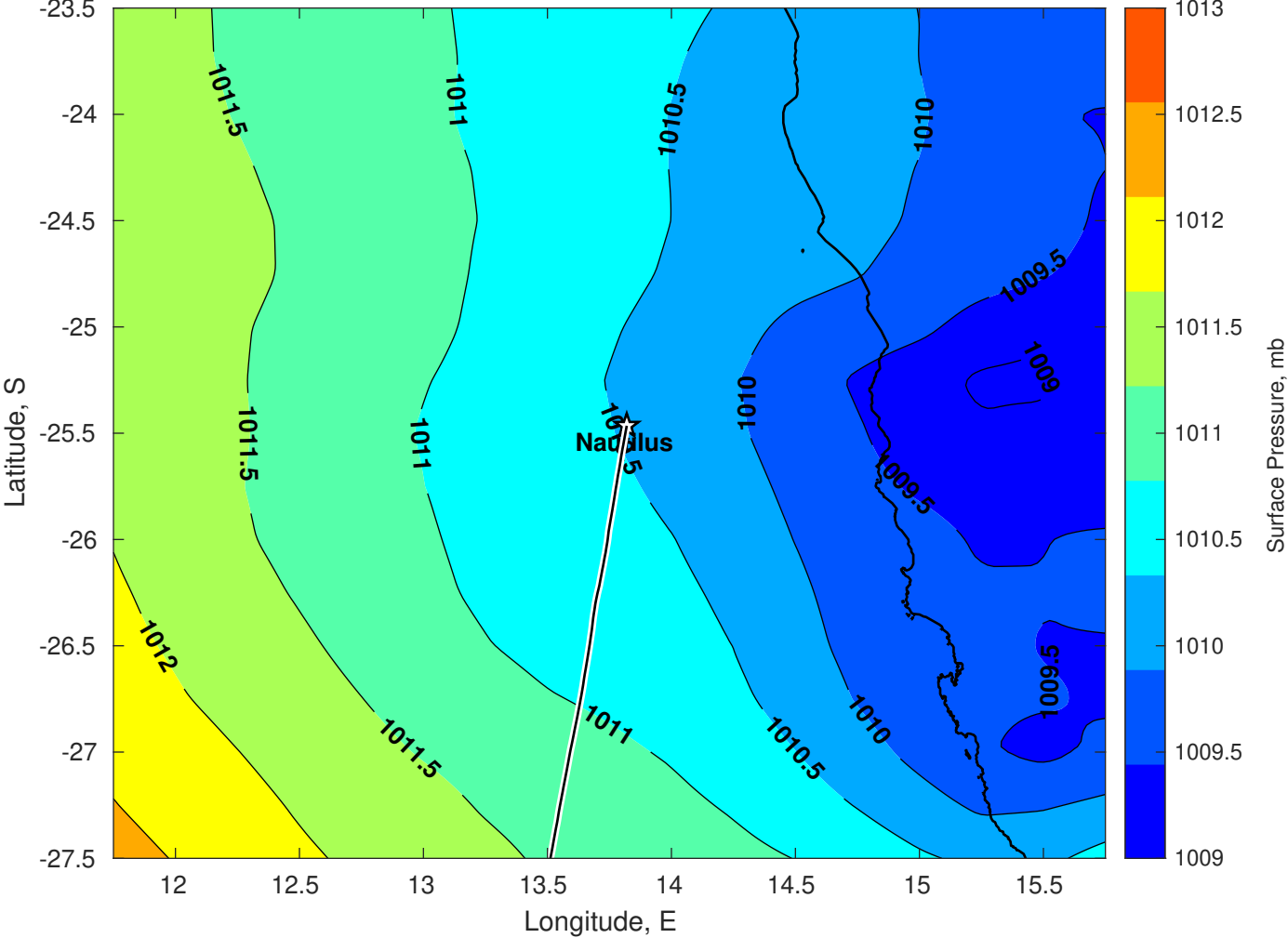
Surface Pressure (mb) for Nautilus at 04-Mar-2025 00:00:00
