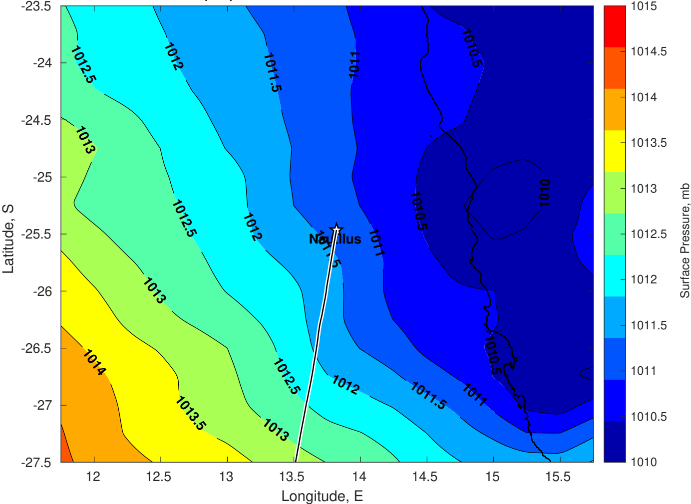
Surface Pressure (mb) for Nautilus at 02-Mar-2025 00:00:00
