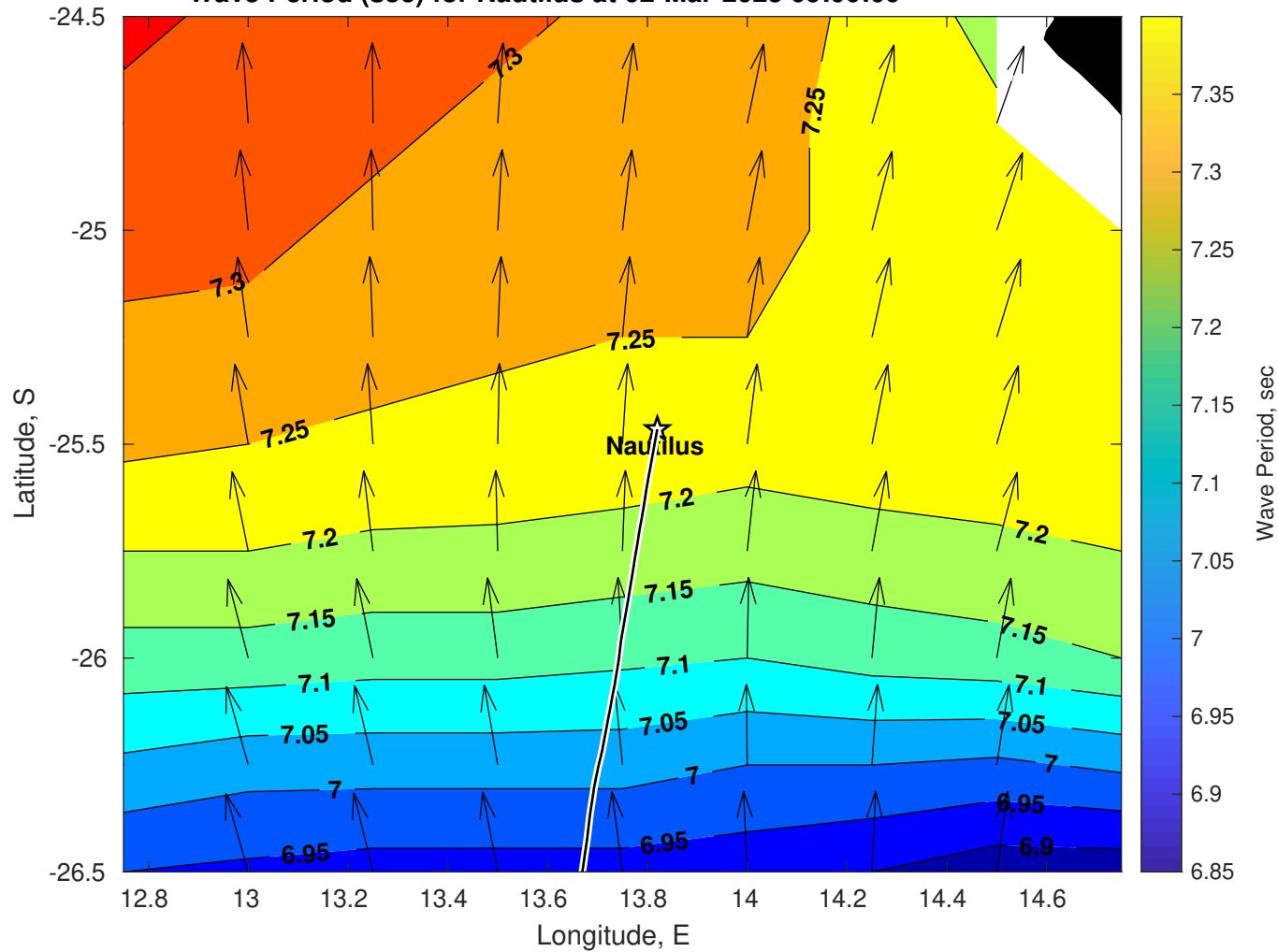
Wave Period (sec) for Nautilus at 02-Mar-2025 09:00:00
