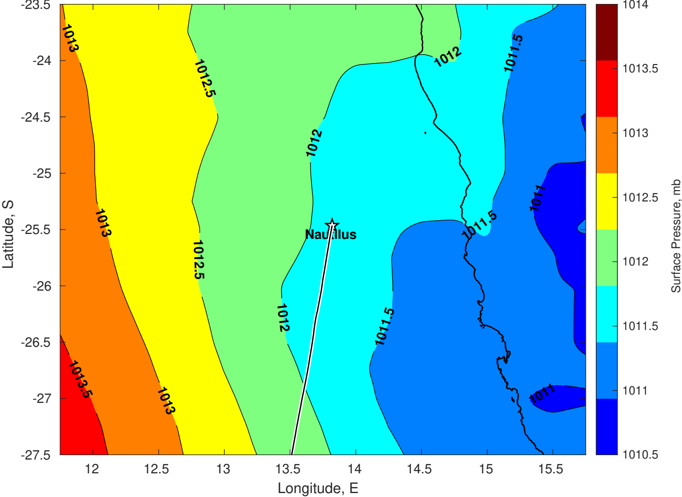
Surface Pressure (mb) for Nautilus at 03-Mar-2025 00:00:00
