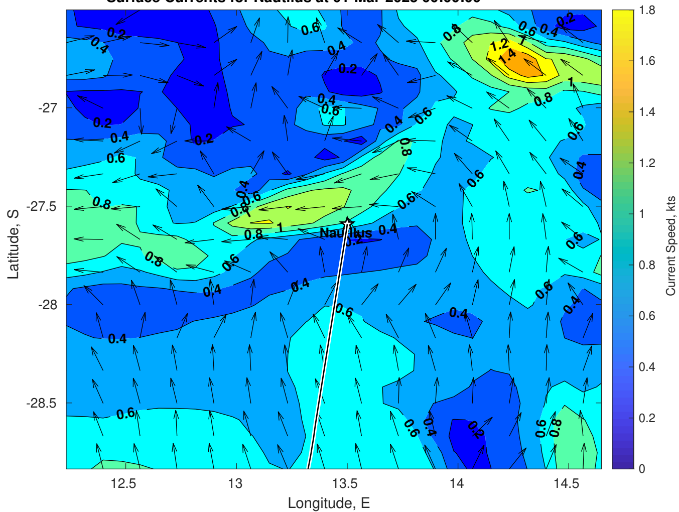
Surface Currents for Nautilus at 01-Mar-2025 00:00:00
