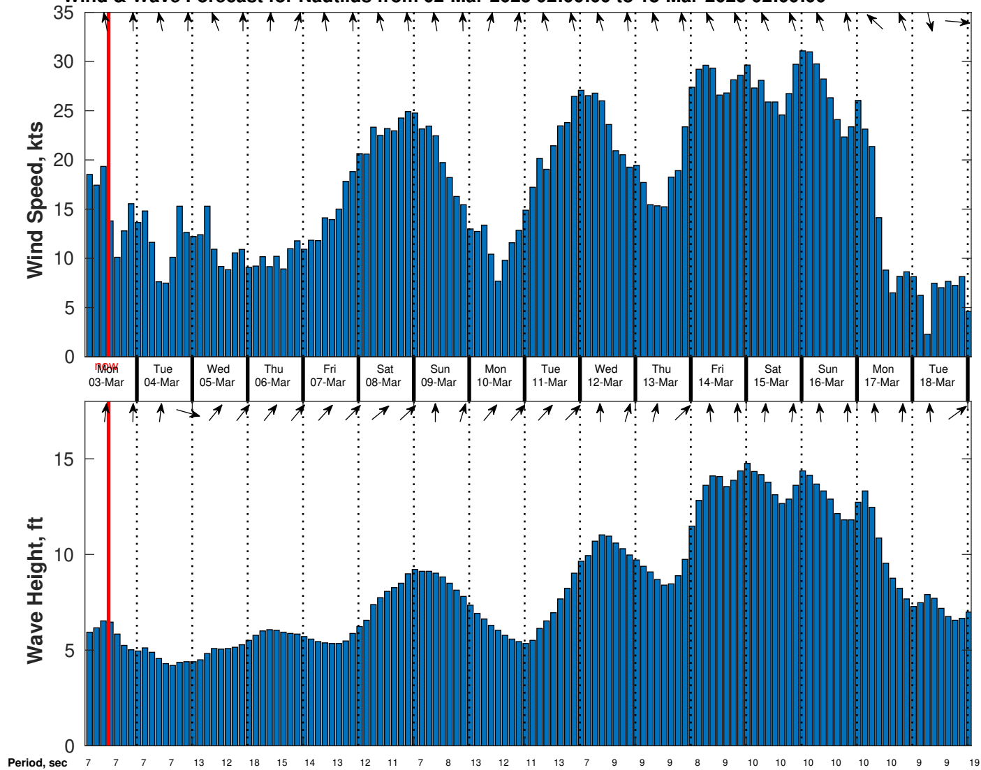
Wind & Wave Forecast for Nautilus from 02-Mar-2025 02:00:00 to 18-Mar-2025 02:00:00
