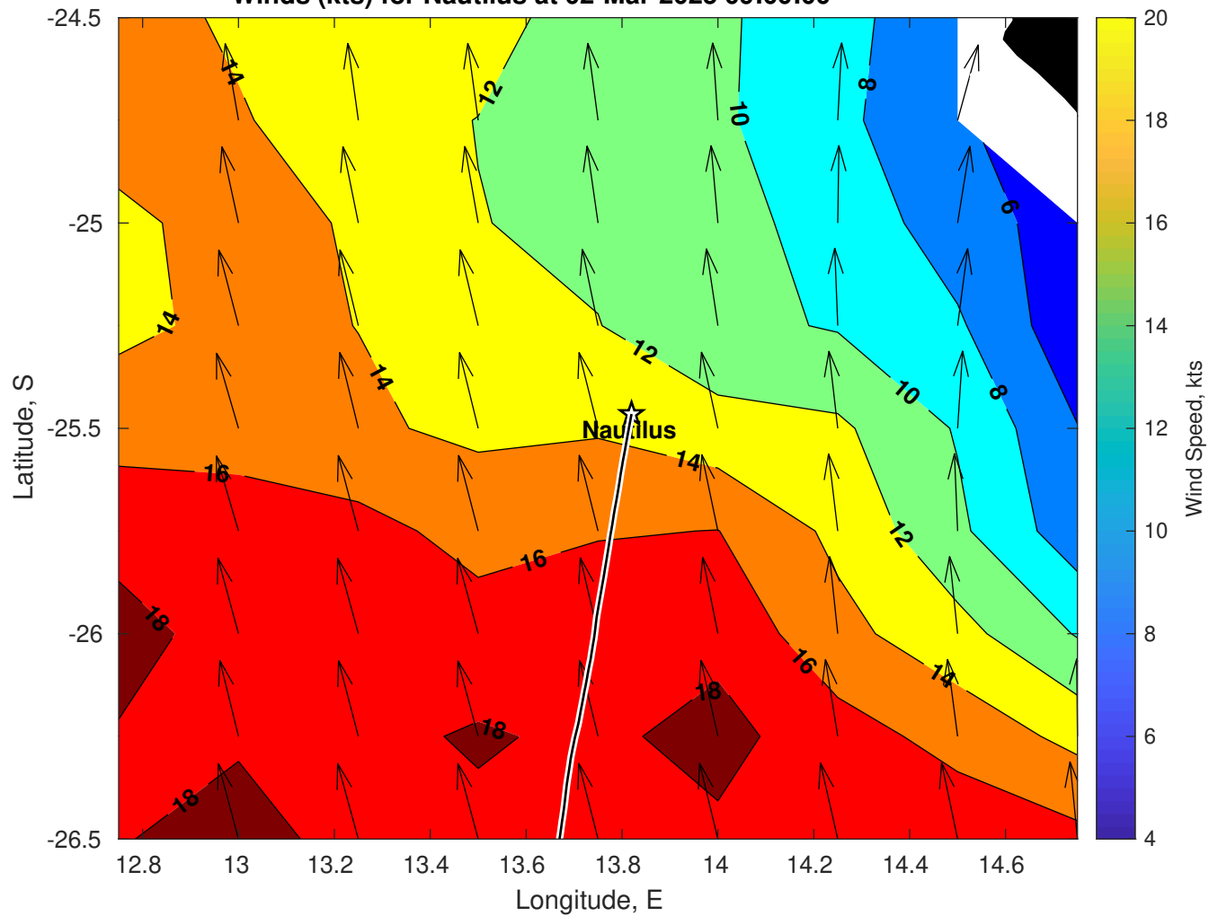
Winds (kts) for Nautilus at 02-Mar-2025 09:00:00
