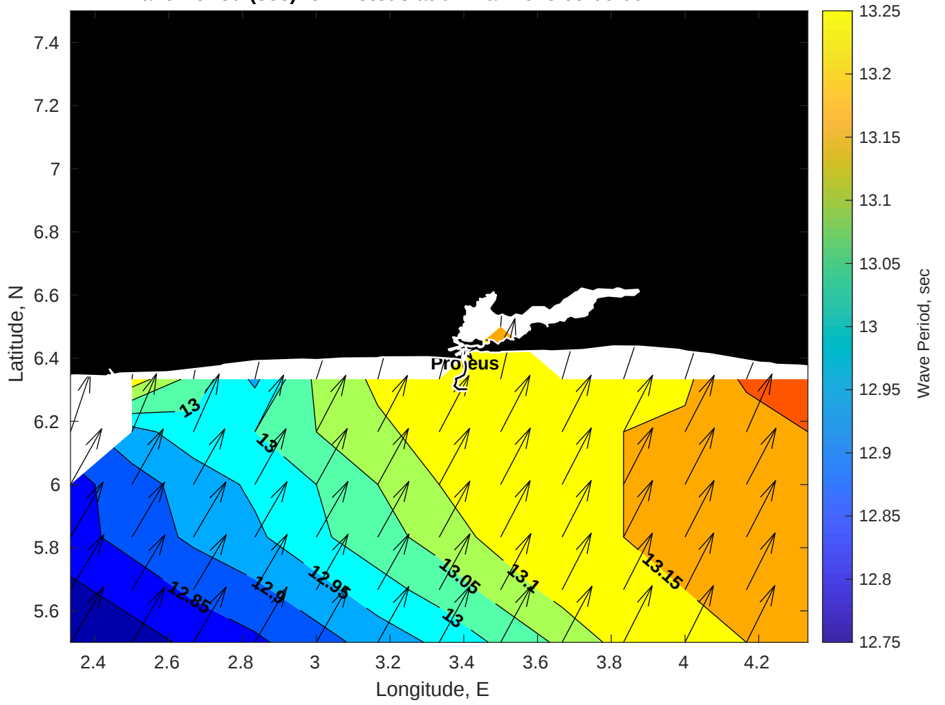
Wave Period (sec) for Proteus at 02-Mar-2025 09:00:00
