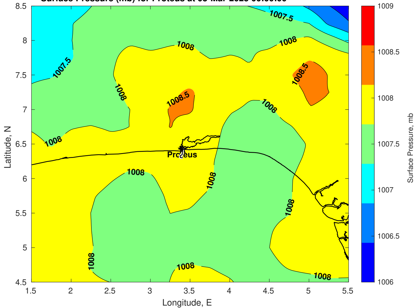
Surface Pressure (mb) for Proteus at 03-Mar-2025 00:00:00
