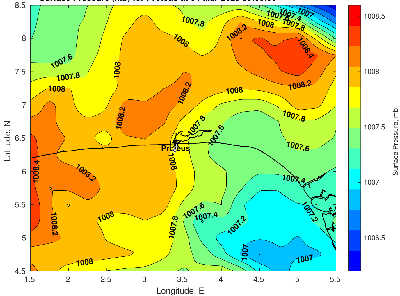
Surface Pressure (mb) for Proteus at 04-Mar-2025 00:00:00
