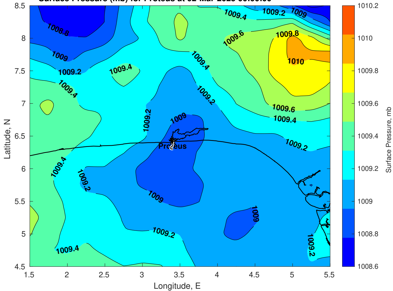
Surface Pressure (mb) for Proteus at 02-Mar-2025 00:00:00
