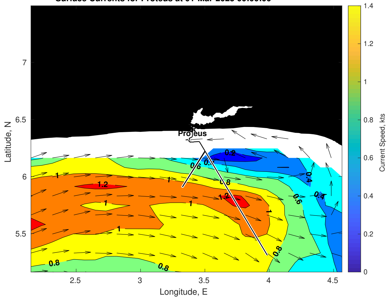
Surface Currents for Proteus at 01-Mar-2025 00:00:00
