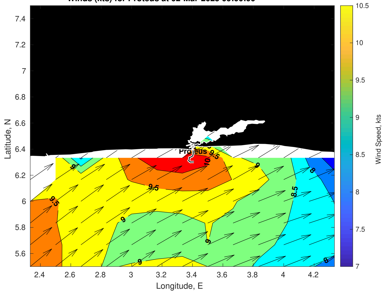
Winds (kts) for Proteus at 02-Mar-2025 09:00:00
