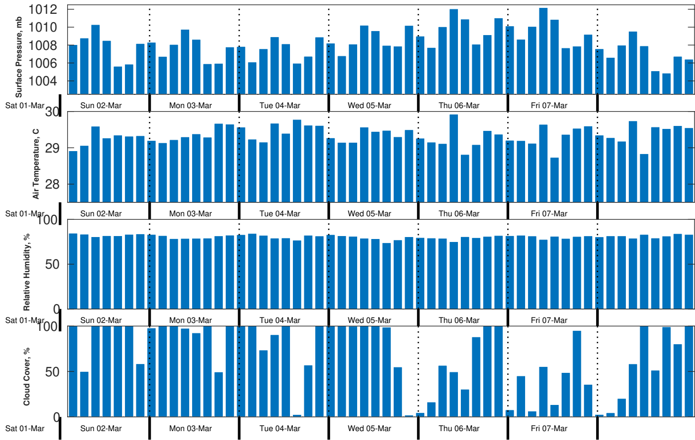
Met Forecast for Proteus from 02-Mar-2025 00:00:00 to 09-Mar-2025 00:00:00
