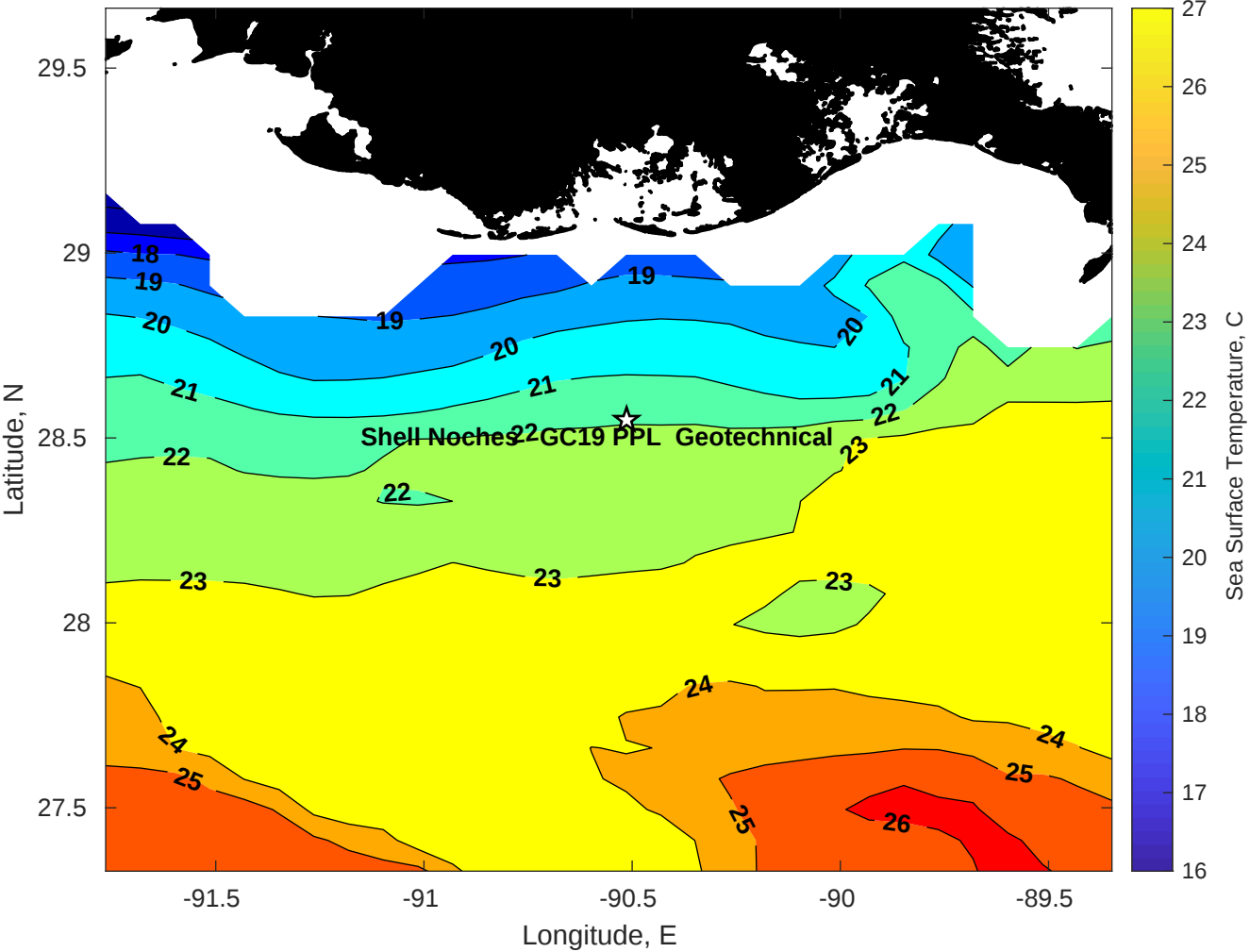
SST for Shell Noches GC19 PPL Geotechnical at 01-Mar-2025 00:00:00
