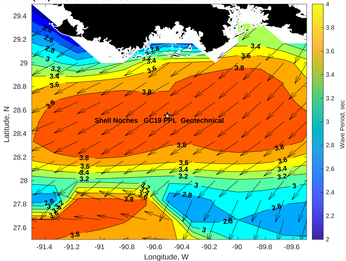
Wave Period (sec) for Shell Noches GC19 PPL Geotechnical at 02-Mar-2025 09:00:00
