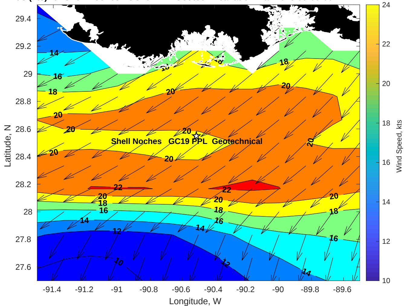
Winds (kts) for Shell Noches GC19 PPL Geotechnical at 02-Mar-2025 09:00:00
