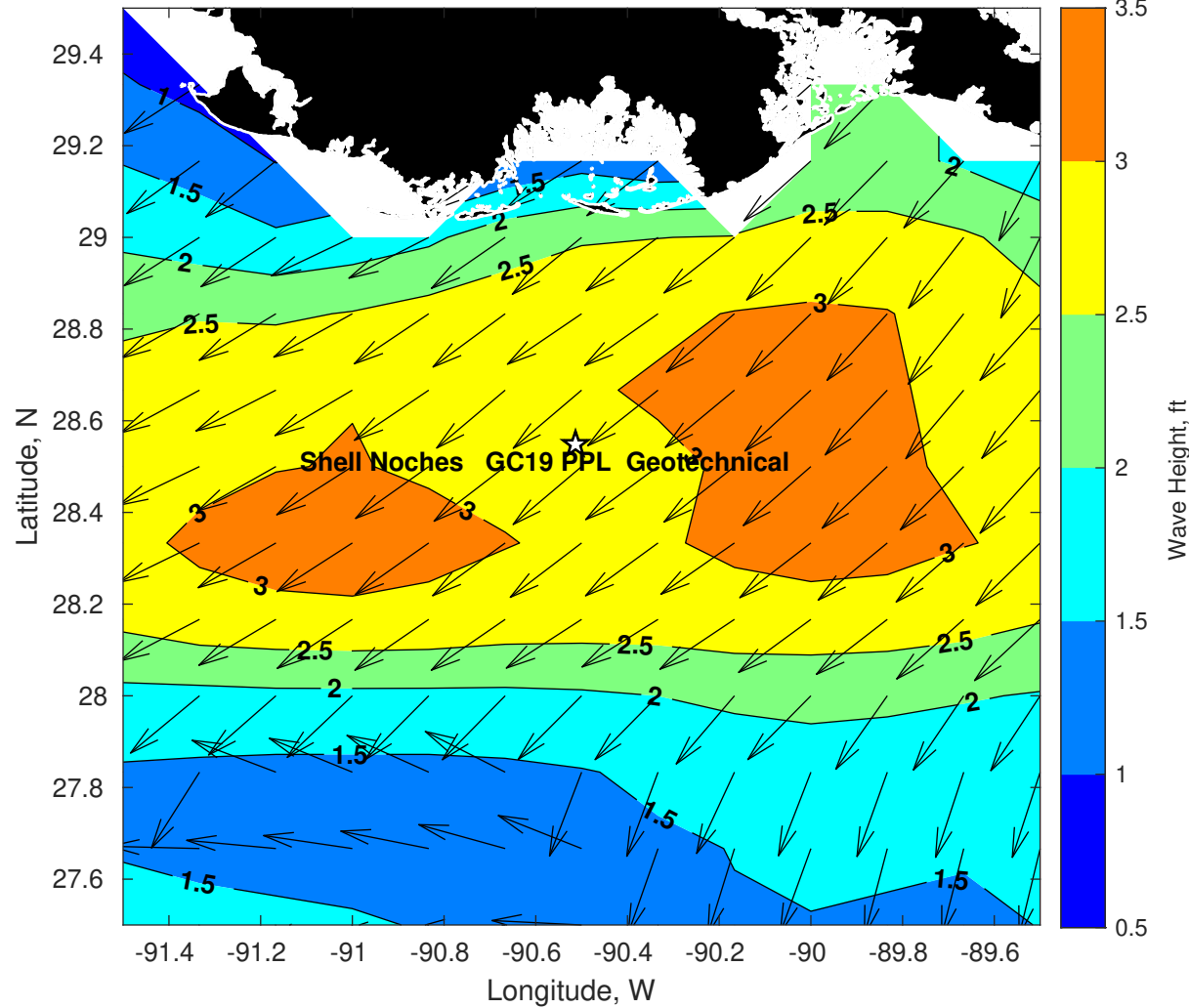
Wave Height (ft) for Shell Noches GC19 PPL Geotechnical at 02-Mar-2025 09:00:00
