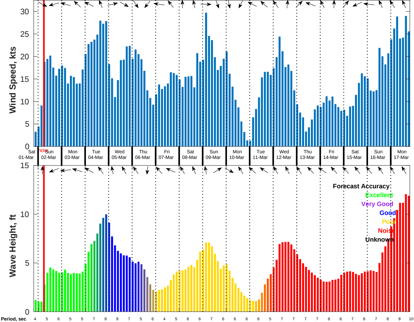
Wind & Wave Forecast for Shell Noches GC19 PPL Geotechnical from 01-Mar-2025 20:00:00 to 17-Mar-2025 20:00:00
