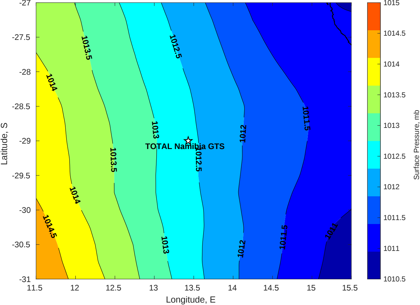
Surface Pressure (mb) for TOTAL Namibia GTS at 03-Mar-2025 00:00:00
