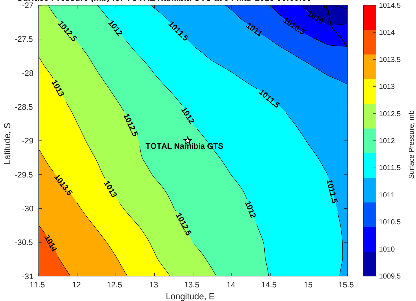
Surface Pressure (mb) for TOTAL Namibia GTS at 04-Mar-2025 00:00:00
