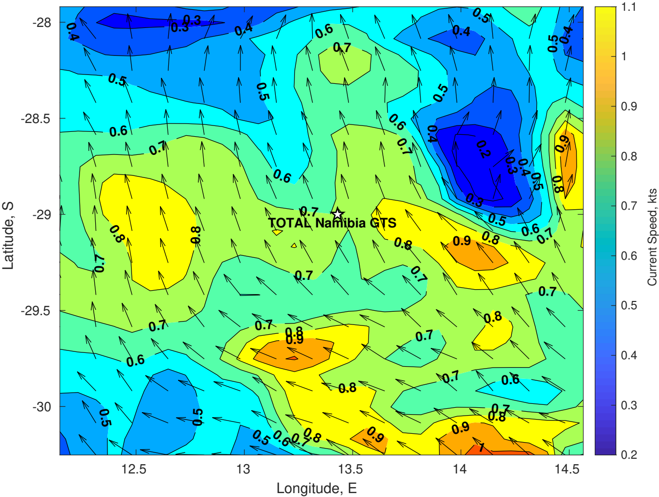
Surface Currents for TOTAL Namibia GTS at 01-Mar-2025 00:00:00
