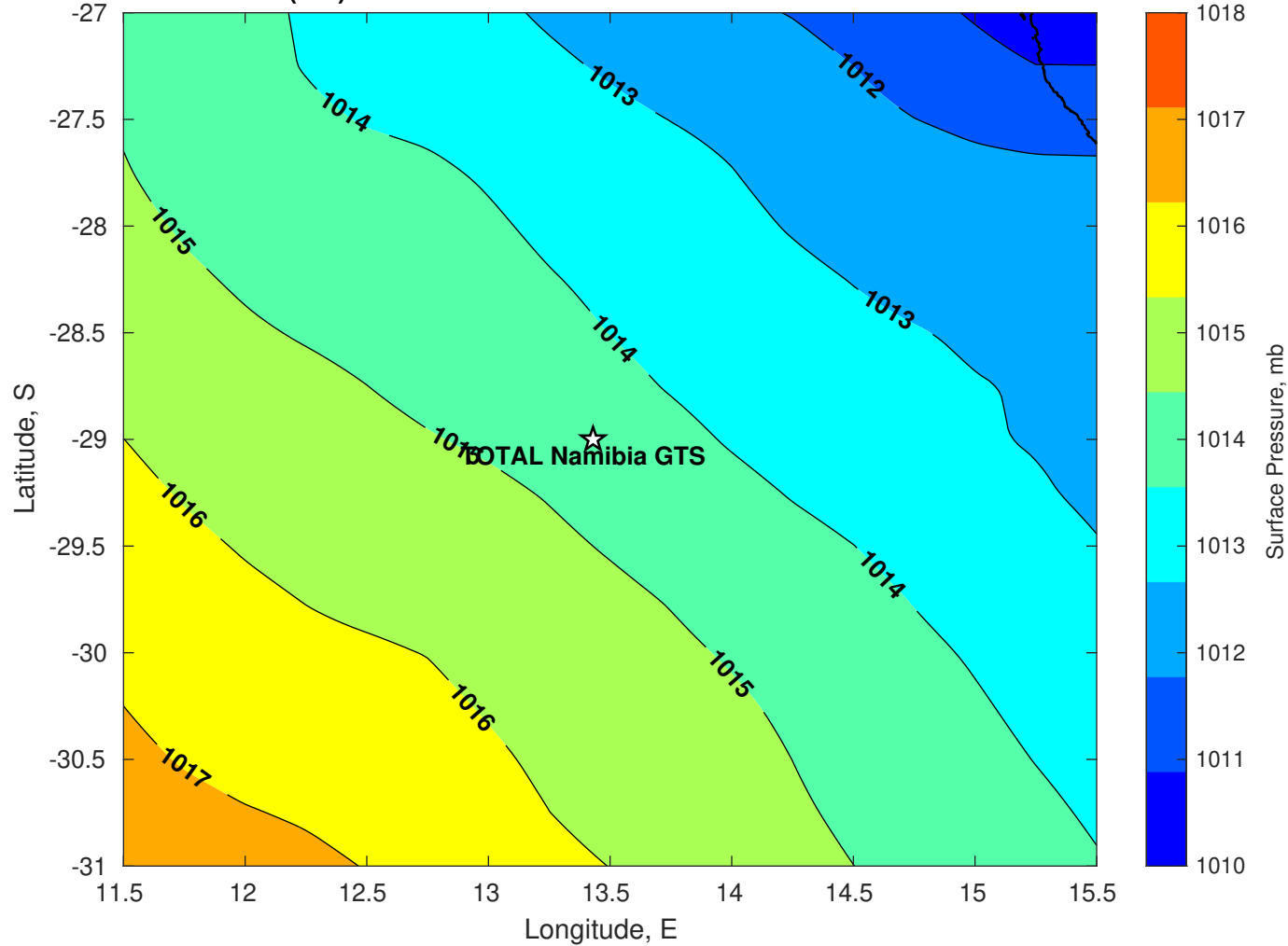
Surface Pressure (mb) for TOTAL Namibia GTS at 02-Mar-2025 00:00:00
