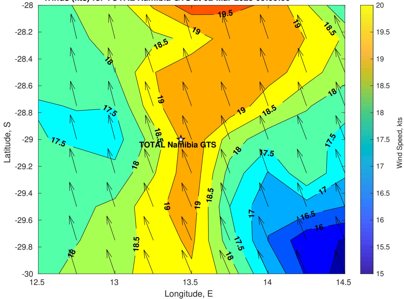
Winds (kts) for TOTAL Namibia GTS at 02-Mar-2025 09:00:00
