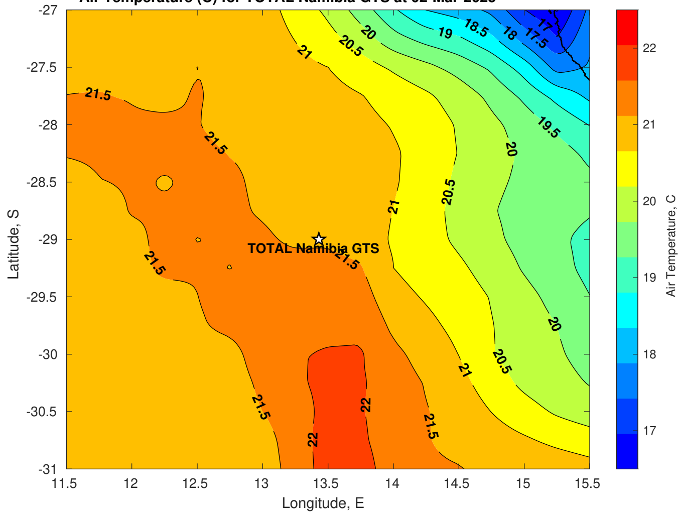
Air Temperature (C) for TOTAL Namibia GTS at 02-Mar-2025
