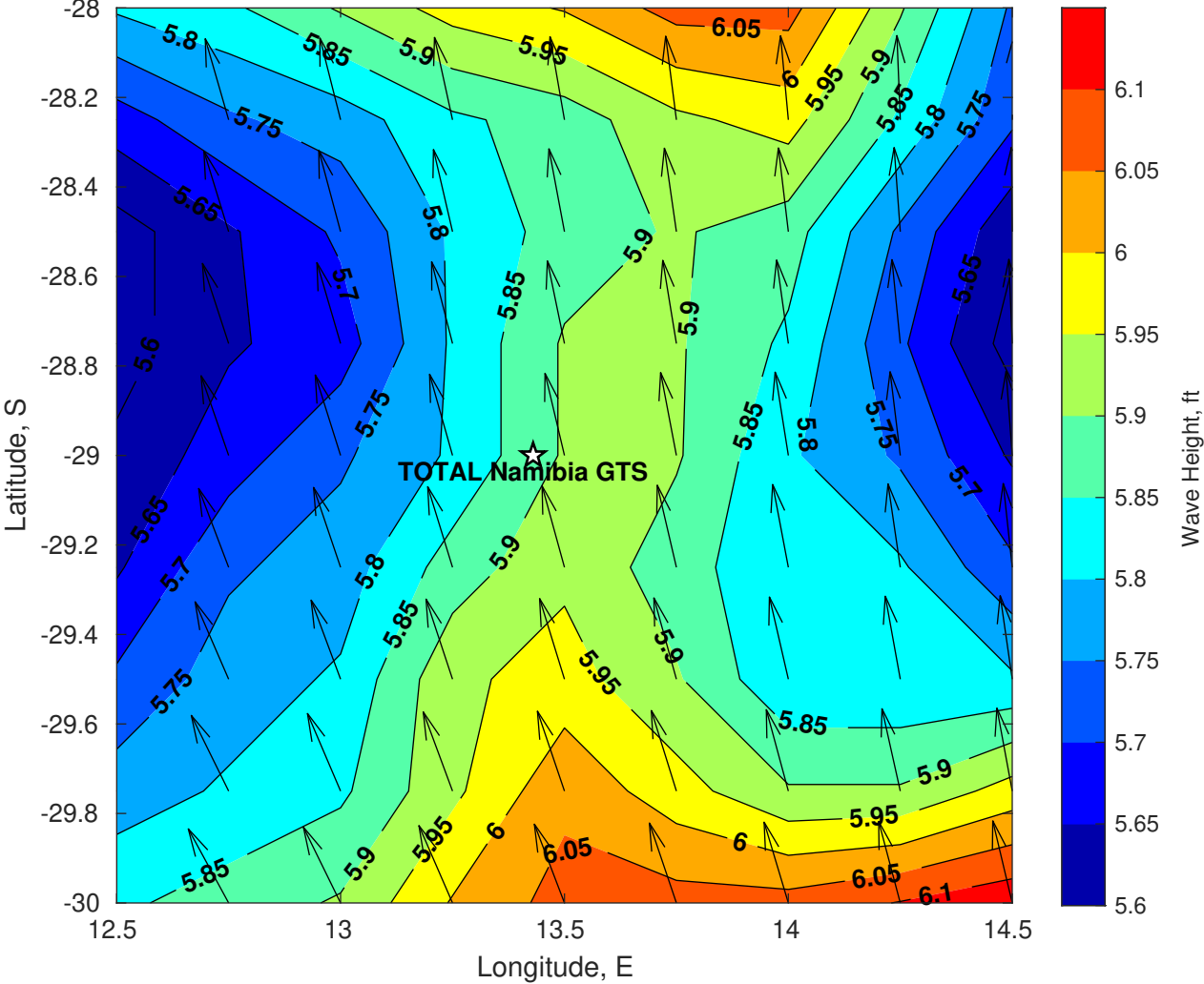
Wave Height (ft) for TOTAL Namibia GTS at 02-Mar-2025 09:00:00
