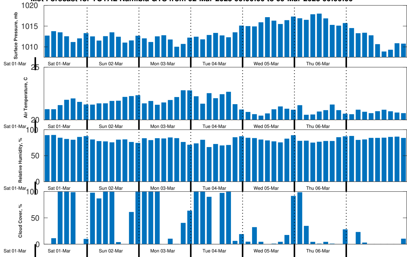
Met Forecast for TOTAL Namibia GTS from 02-Mar-2025 00:00:00 to 09-Mar-2025 00:00:00
