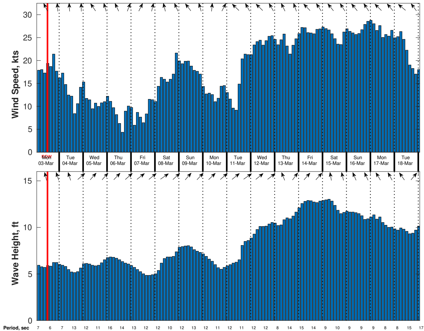
Wind & Wave Forecast for TOTAL Namibia GTS from 02-Mar-2025 02:00:00 to 18-Mar-2025 02:00:00
