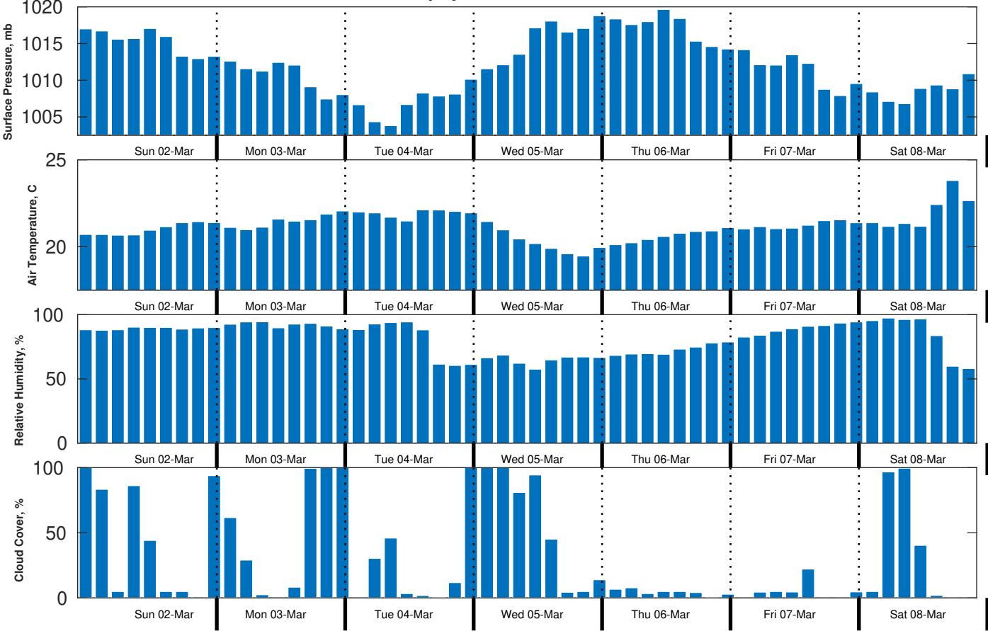
Met Forecast for Tampnet P2378 South Texas Cable Route Geophysical from 02-Mar-2025 00:00:00 to 09-Mar-2025 00:00:00
