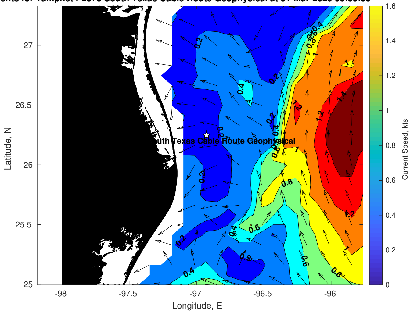
Surface Currents for Tampnet P2378 South Texas Cable Route Geophysical at 01-Mar-2025 00:00:00
