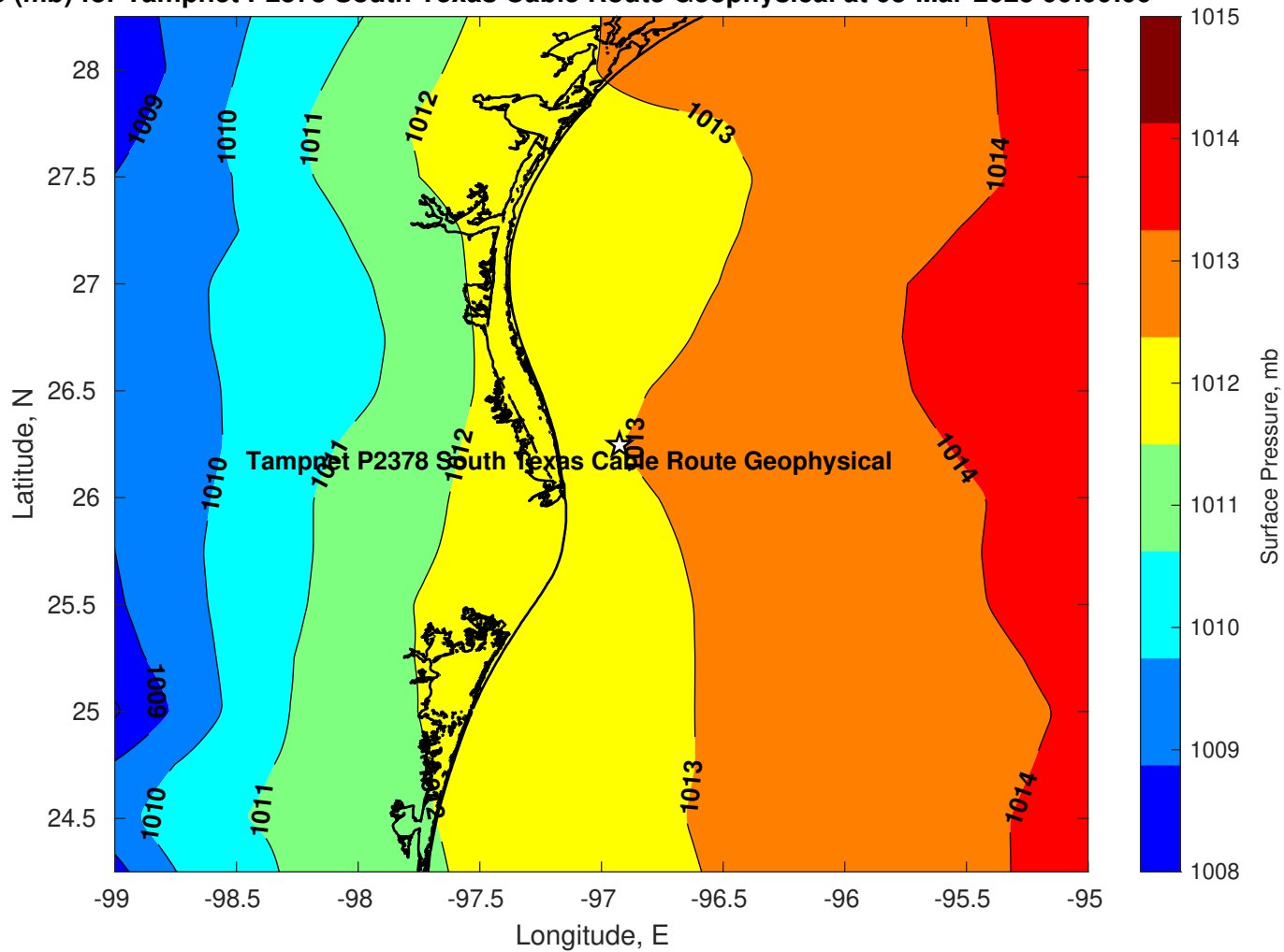
Pressure (mb) for Tampnet P2378 South Texas Cable Route Geophysical at 03-Mar-2025 00:00:00
