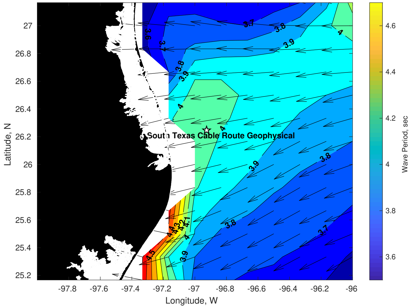
Period (sec) for Tampnet P2378 South Texas Cable Route Geophysical at 02-Mar-2025 09:00:00
