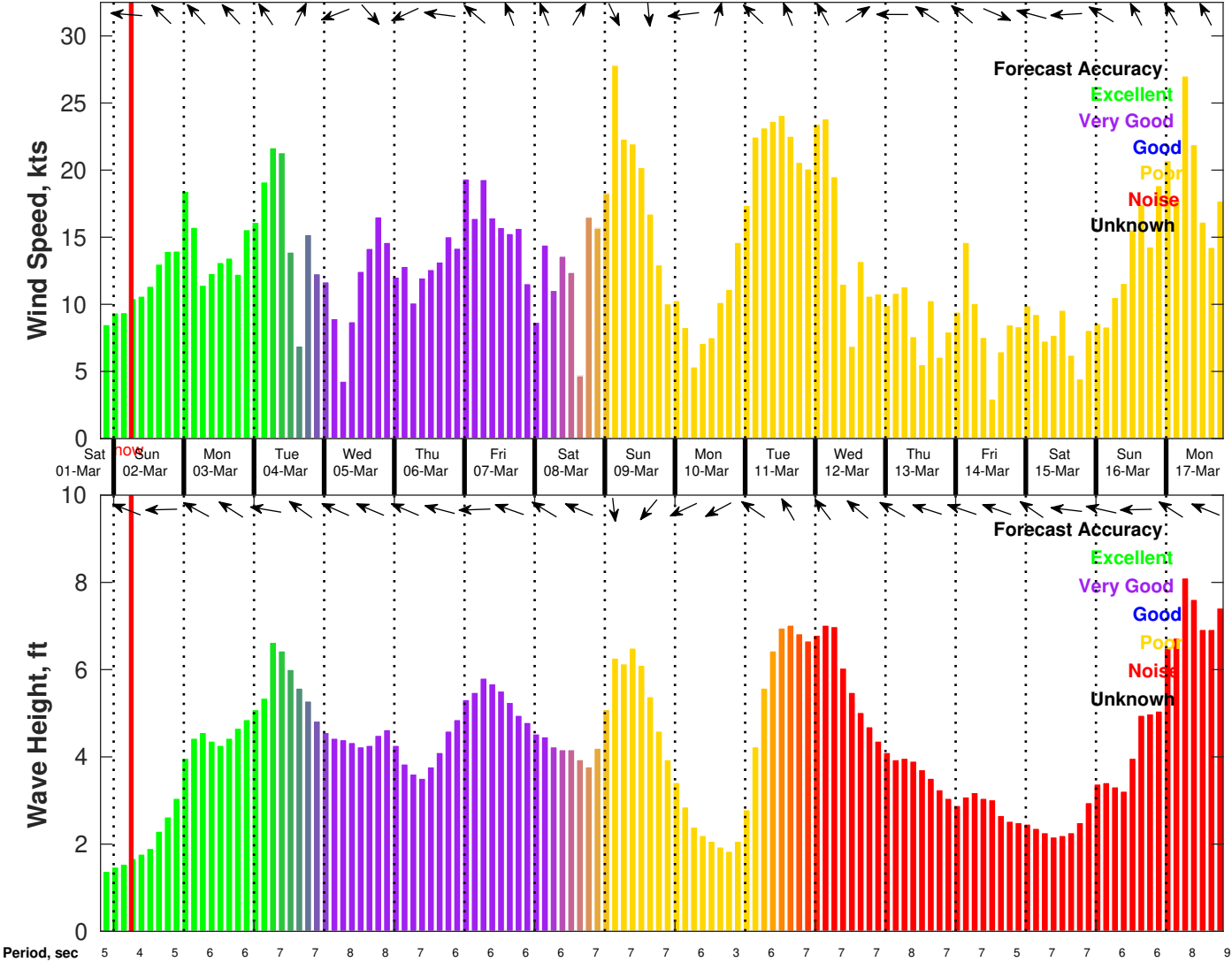
Wind & Wave Forecast for Tampnet P2378 South Texas Cable Route Geophysical from 01-Mar-2025 20:00:00 to 17-Mar-2025 20:00:00
