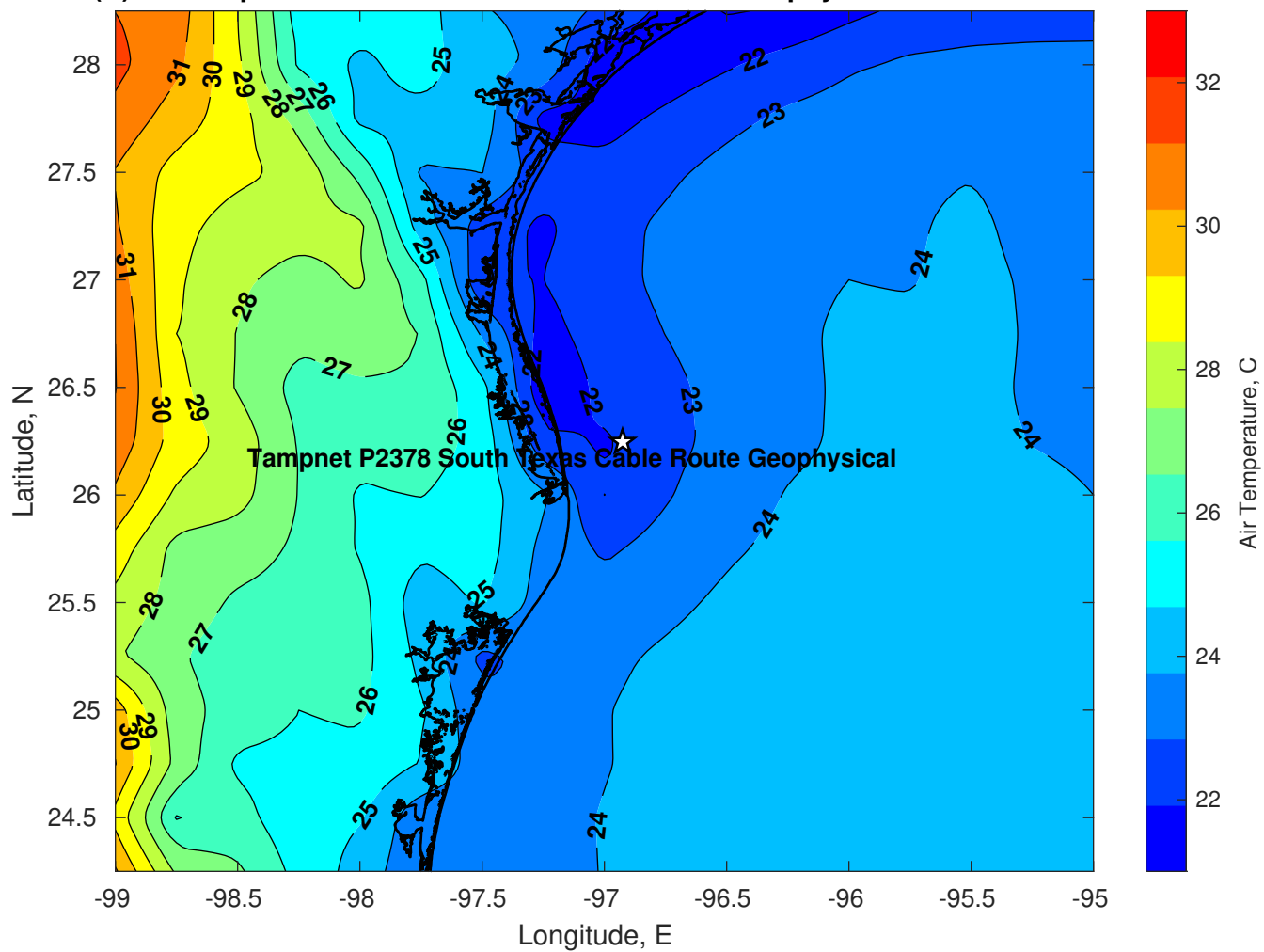
Air Temperature (C) for Tampnet P2378 South Texas Cable Route Geophysical at 02-Mar-2025
