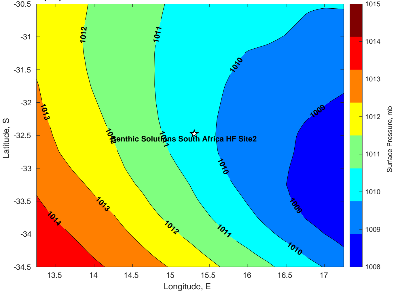
Surface Pressure (mb) for Benthic Solutions South Africa HF Site2 at 03-Mar-2025 00:00:00
