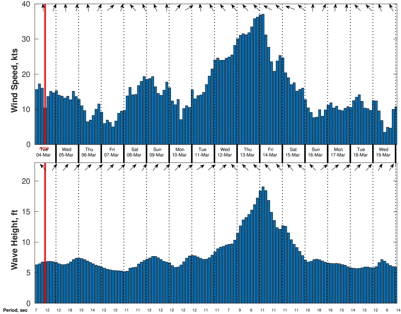
Wind & Wave Forecast for Benthic Solutions South Africa HF Site2 from 03-Mar-2025 02:00:00 to 19-Mar-2025 02:00:00
