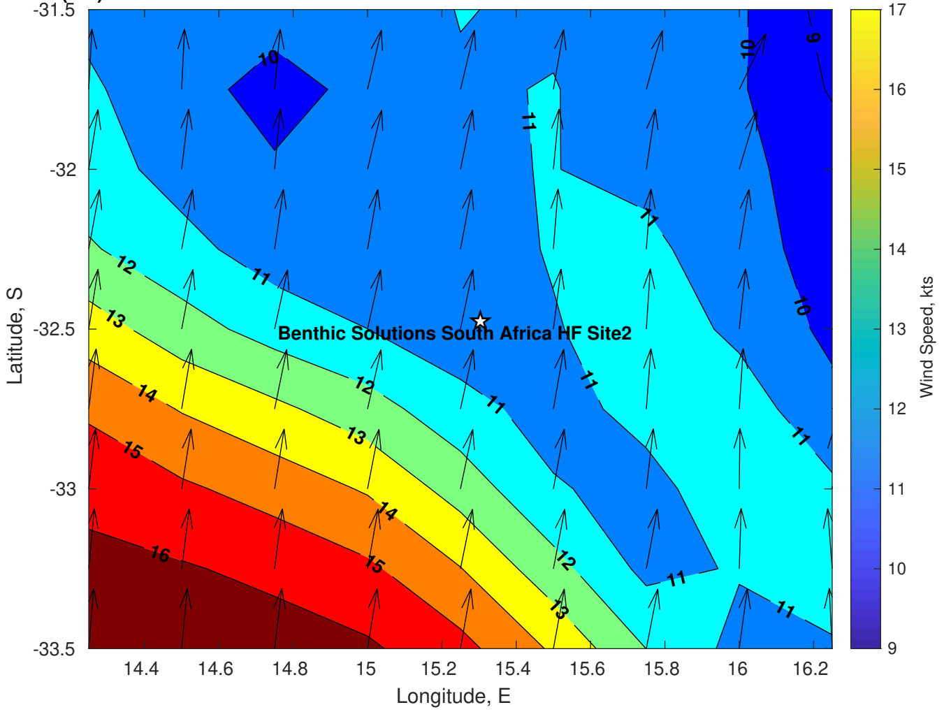
Winds (kts) for Benthic Solutions South Africa HF Site2 at 03-Mar-2025 09:00:00
