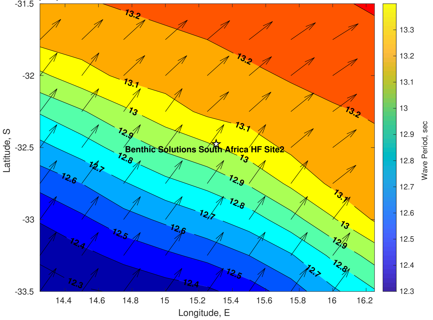
Wave Period (sec) for Benthic Solutions South Africa HF Site2 at 03-Mar-2025 09:00:00
