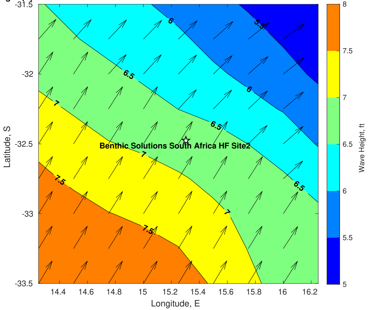
Wave Height (ft) for Benthic Solutions South Africa HF Site2 at 03-Mar-2025 09:00:00
