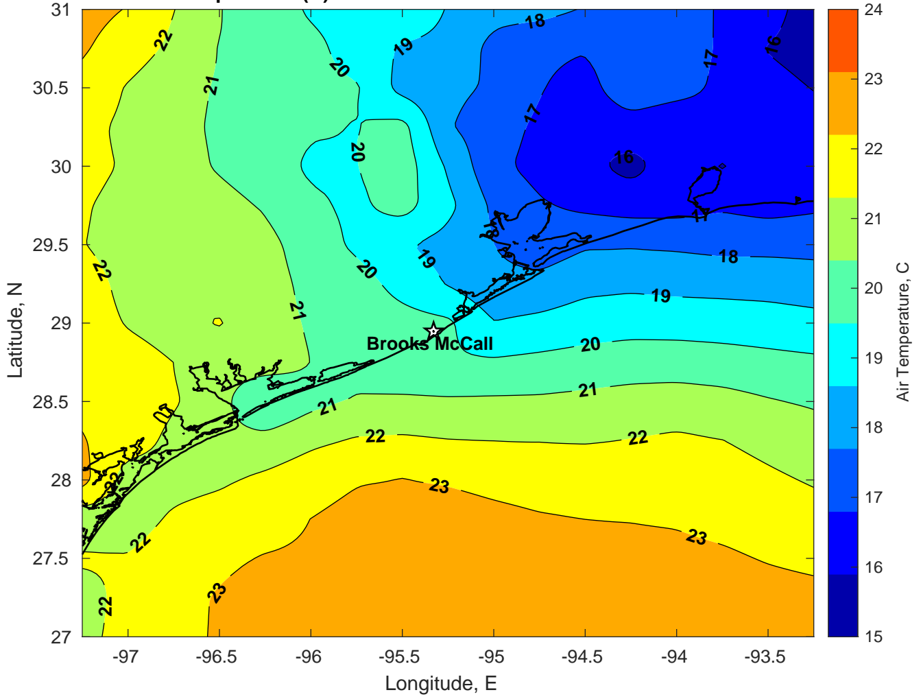
Air Temperature (C) for Brooks McCall at 03-Mar-2025
