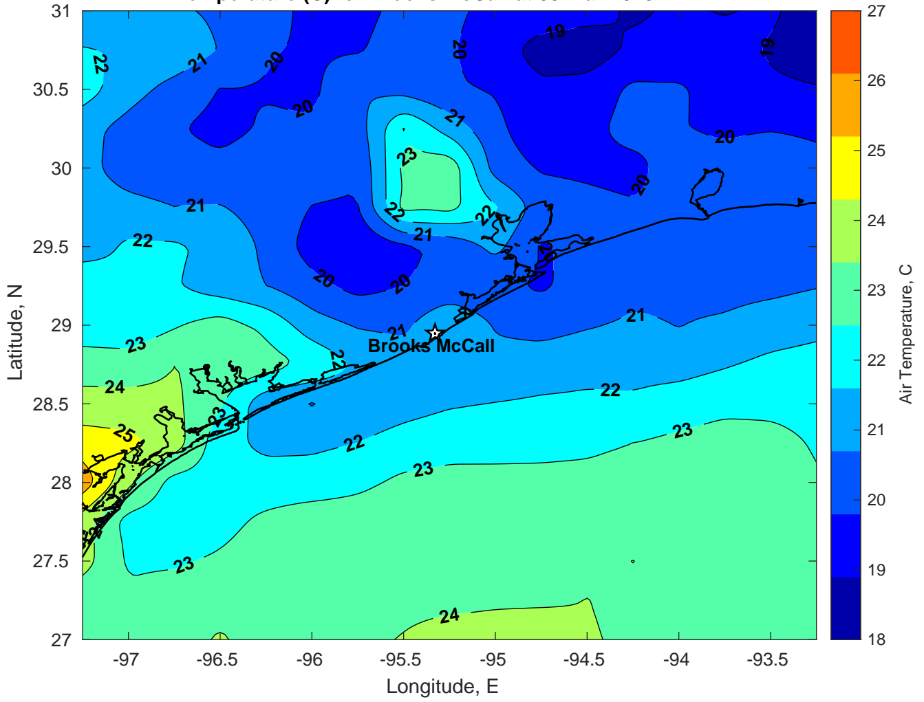
Air Temperature (C) for Brooks McCall at 03-Mar-2025
