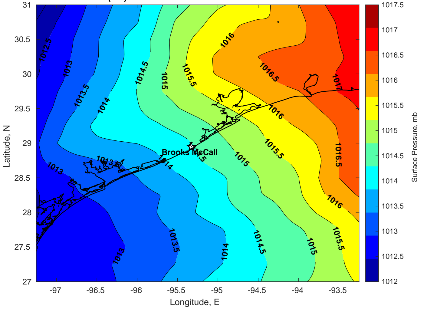
Surface Pressure (mb) for Brooks McCall at 03-Mar-2025 00:00:00
