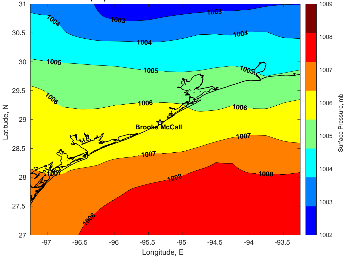
Surface Pressure (mb) for Brooks McCall at 05-Mar-2025 00:00:00
