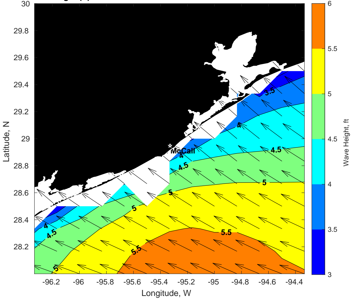
Wave Height (ft) for Brooks McCall at 03-Mar-2025 09:00:00
