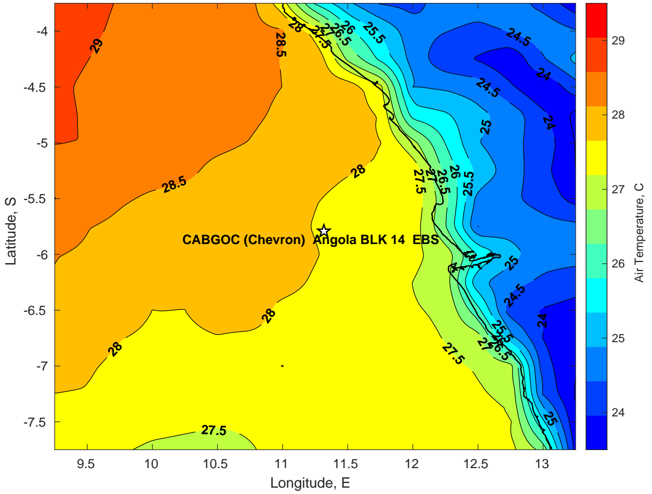
Air Temperature (C) for CABGOC (Chevron) Angola BLK 14 EBS at 03-Mar-2025
