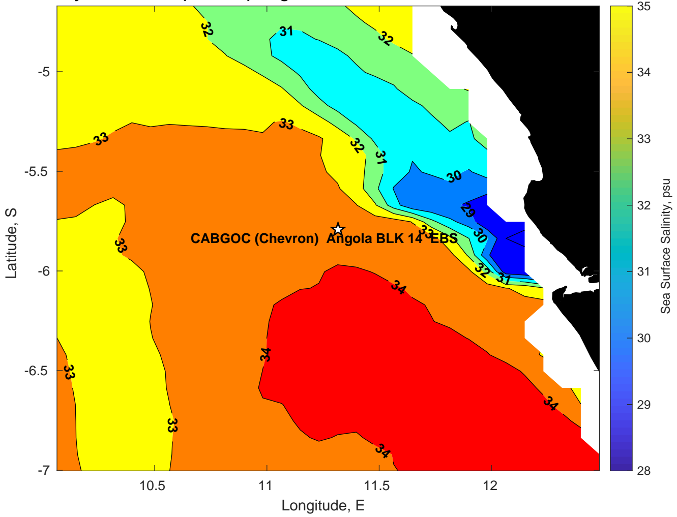
Surface Salinity for CABGOC (Chevron) Angola BLK 14 EBS at 02-Mar-2025 00:00:00
