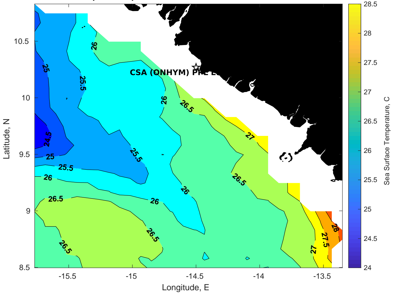
SST for CSA (ONHYM) PPL EBS - Guinea at 02-Mar-2025 00:00:00
