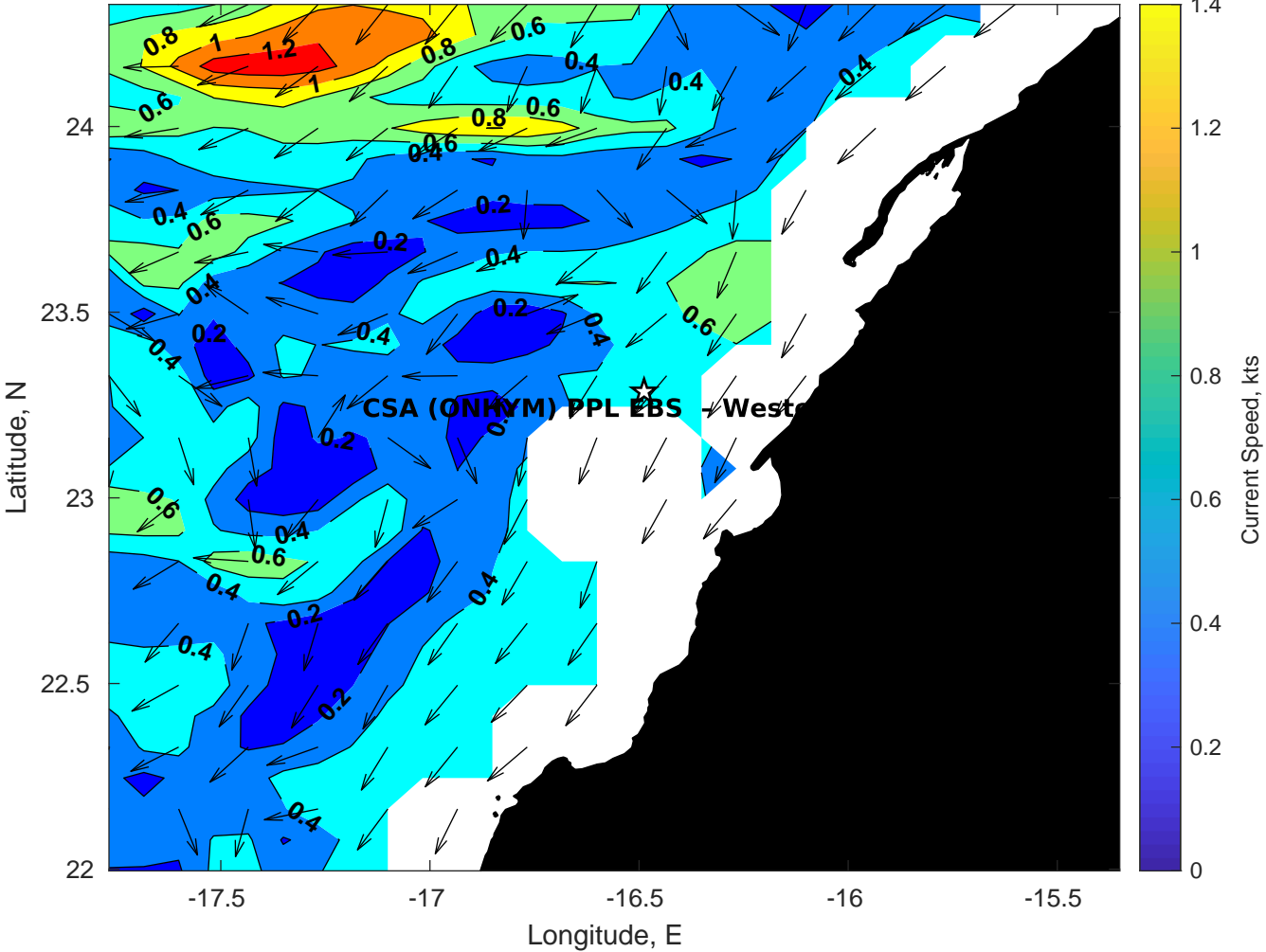
Surface Currents for CSA (ONHYM) PPL EBS - Western Sahara at 02-Mar-2025 00:00:00
