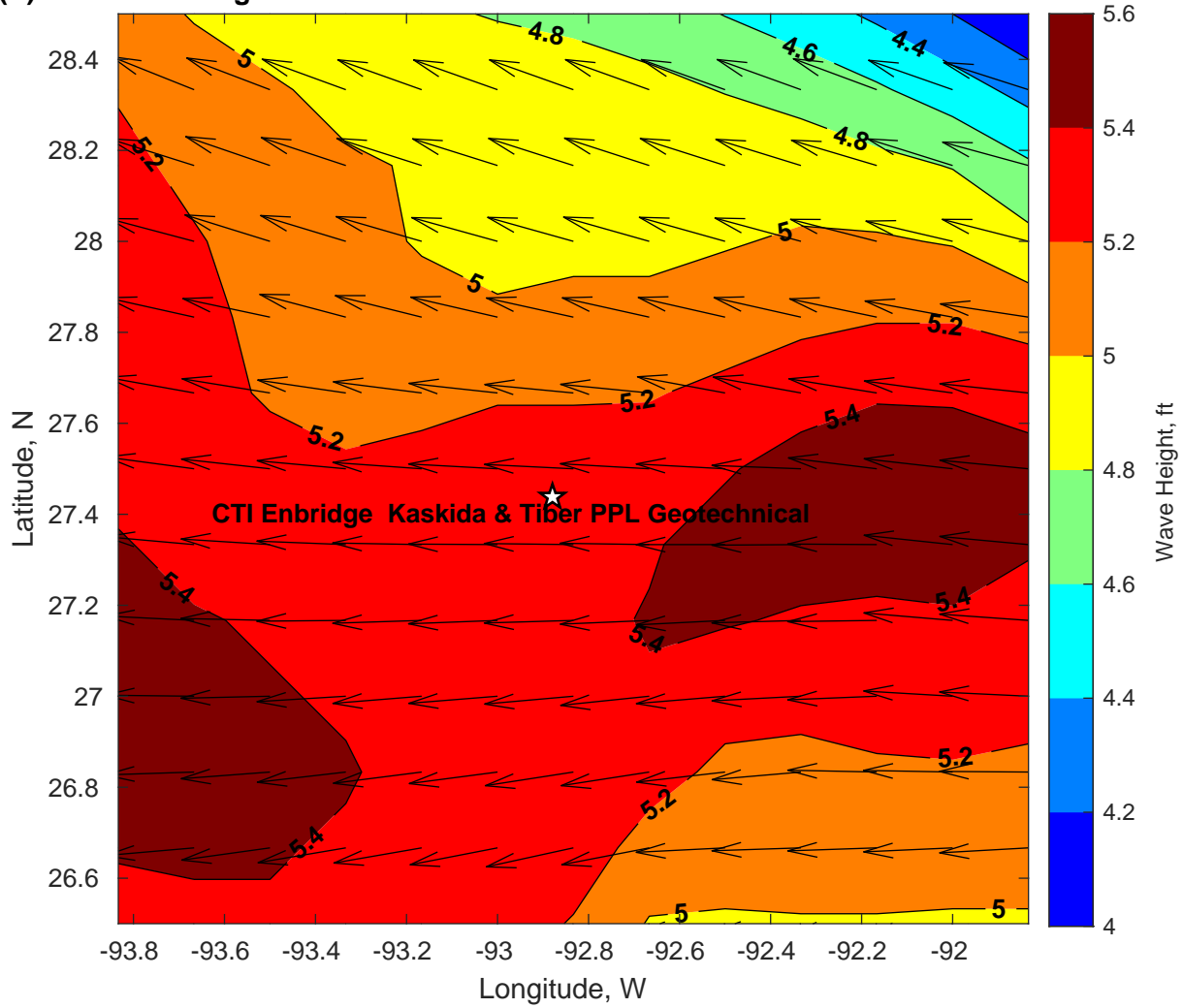
Wave Height (ft) for CTI Enbridge Kaskida & Tiber PPL Geotechnical at 03-Mar-2025 09:00:00
