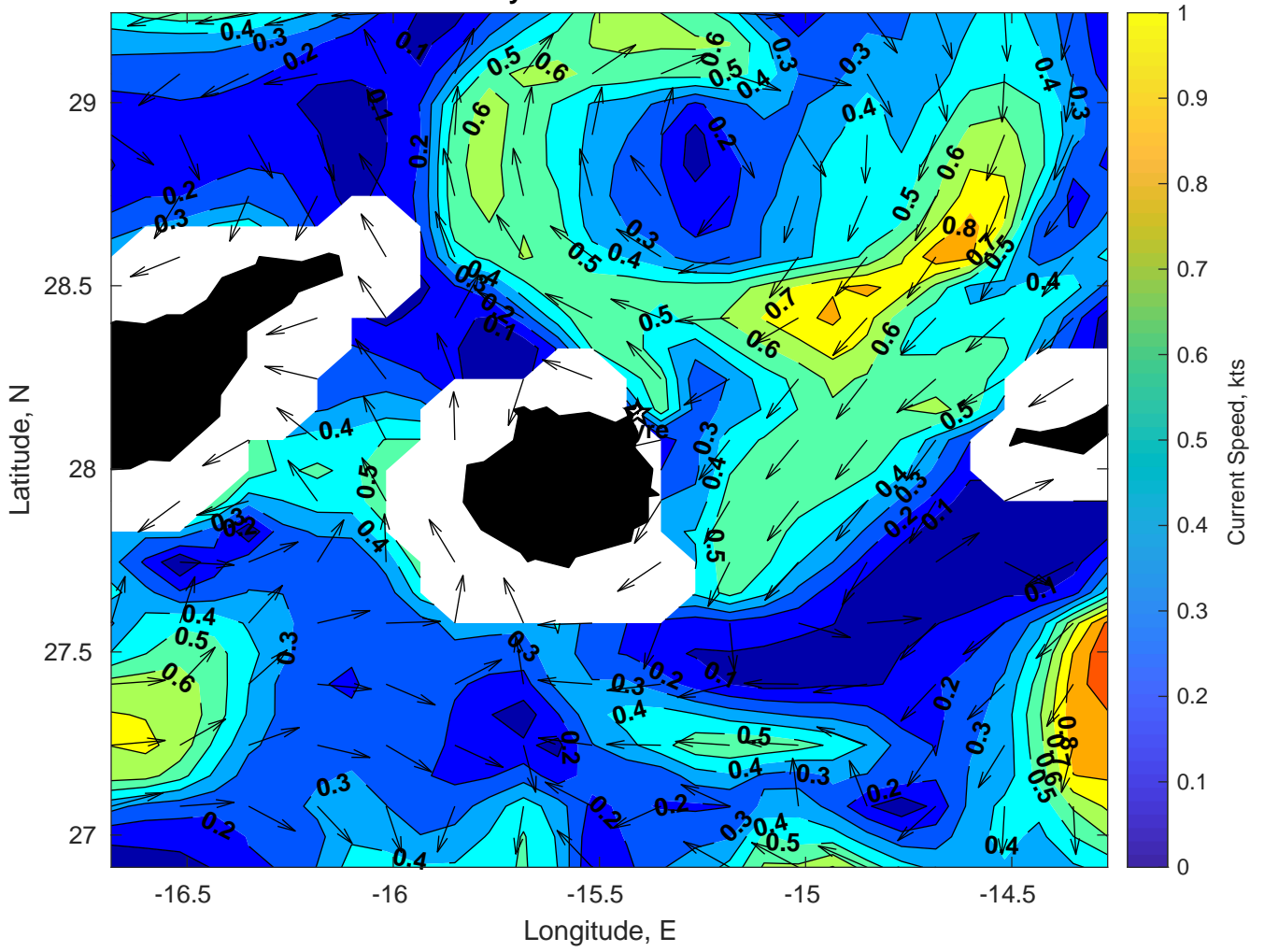
Surface Currents for Gyre at 02-Mar-2025 00:00:00
