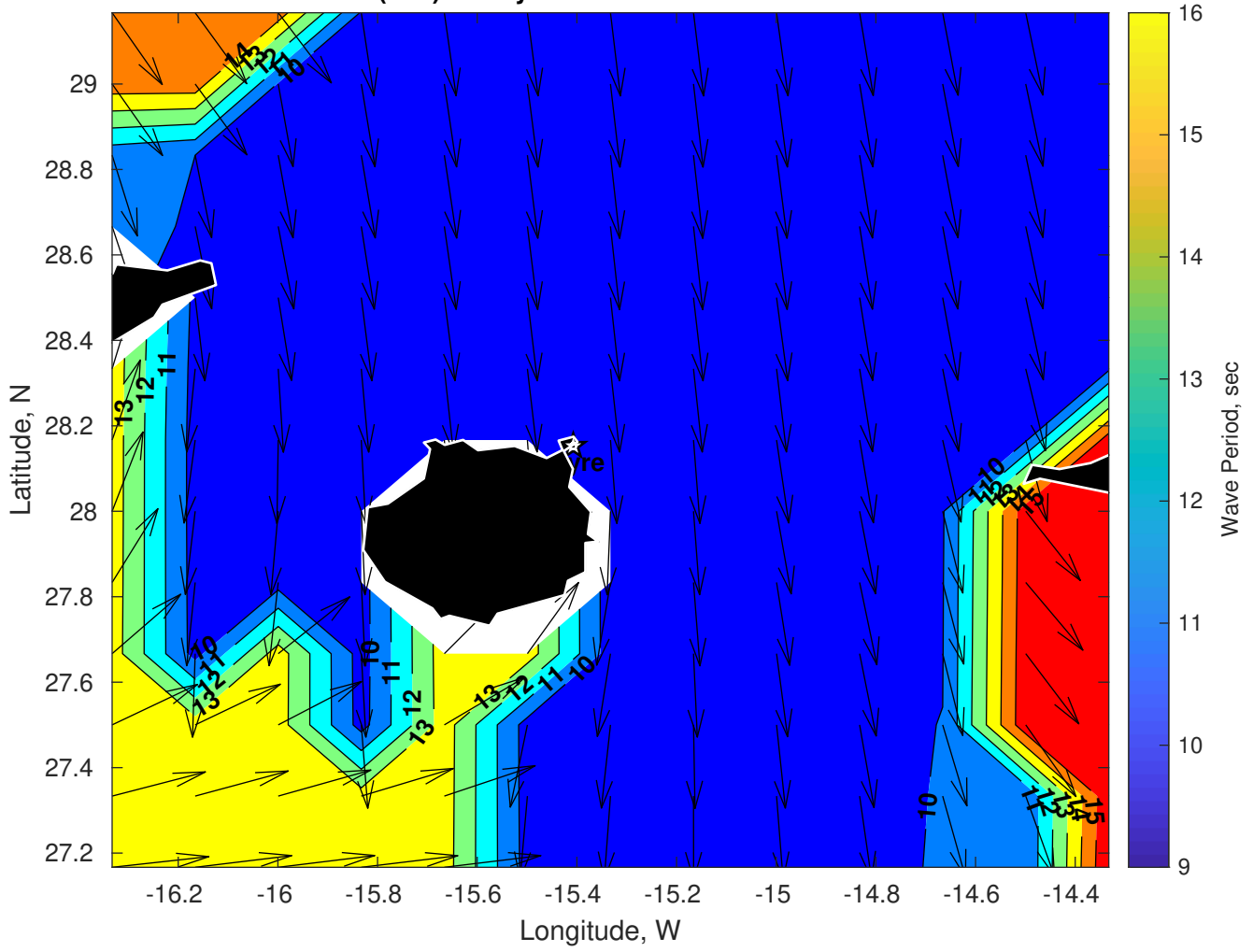
Wave Period (sec) for Gyre at 03-Mar-2025 09:00:00
