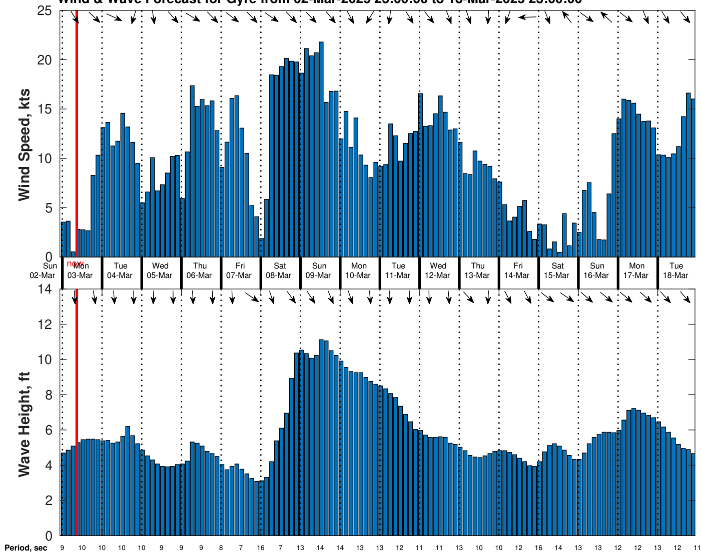
Wind & Wave Forecast for Gyre from 02-Mar-2025 23:00:00 to 18-Mar-2025 23:00:00
