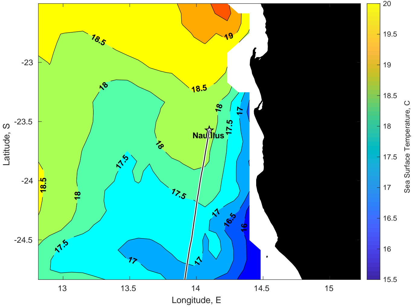
SST for Nautilus at 02-Mar-2025 00:00:00
