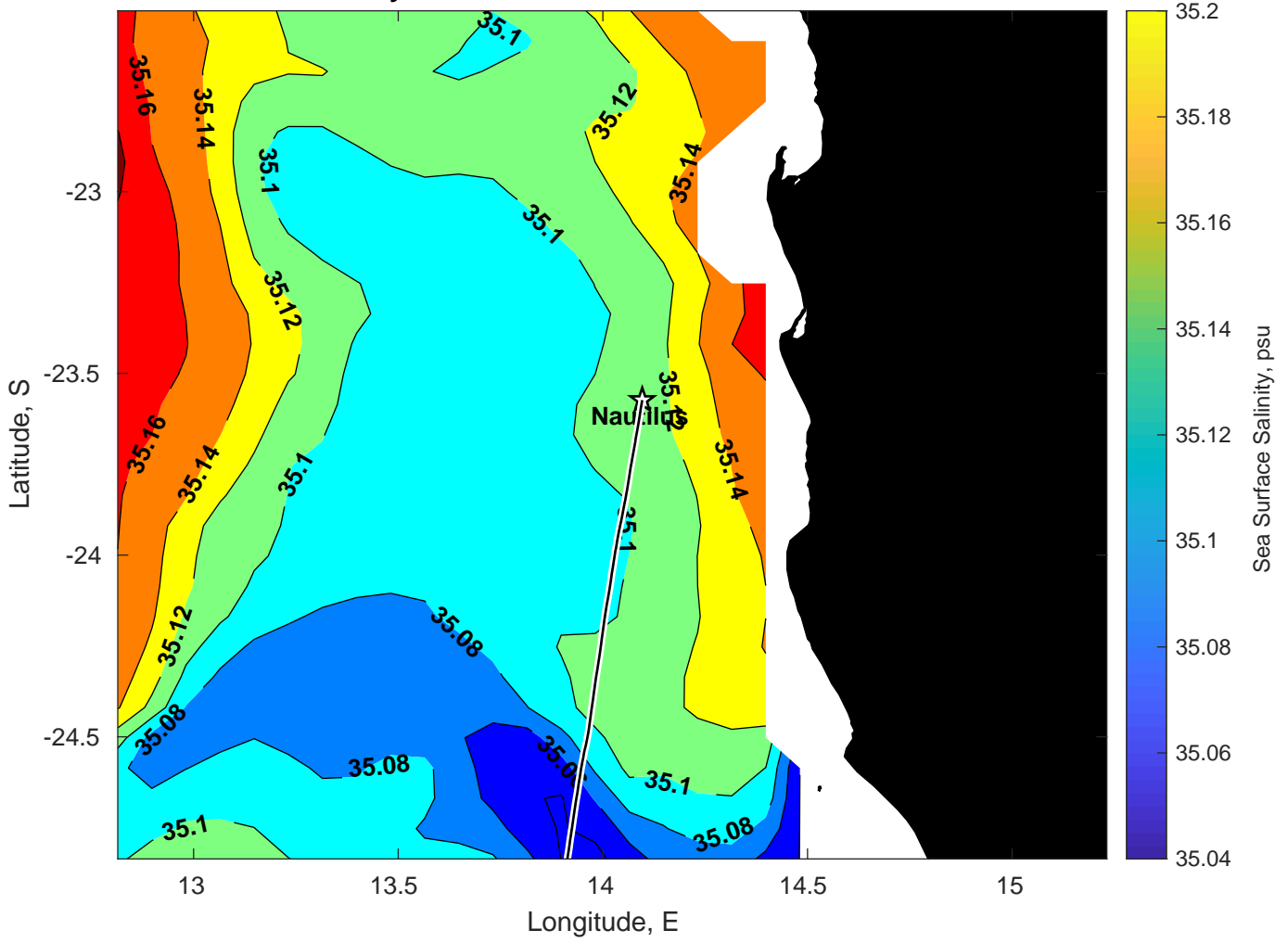
Surface Salinity for Nautilus at 02-Mar-2025 00:00:00
