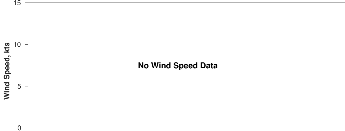
Wind & Wave Forecast for Nautilus from 03-Mar-2025 02:00:00 to 19-Mar-2025 02:00:00
