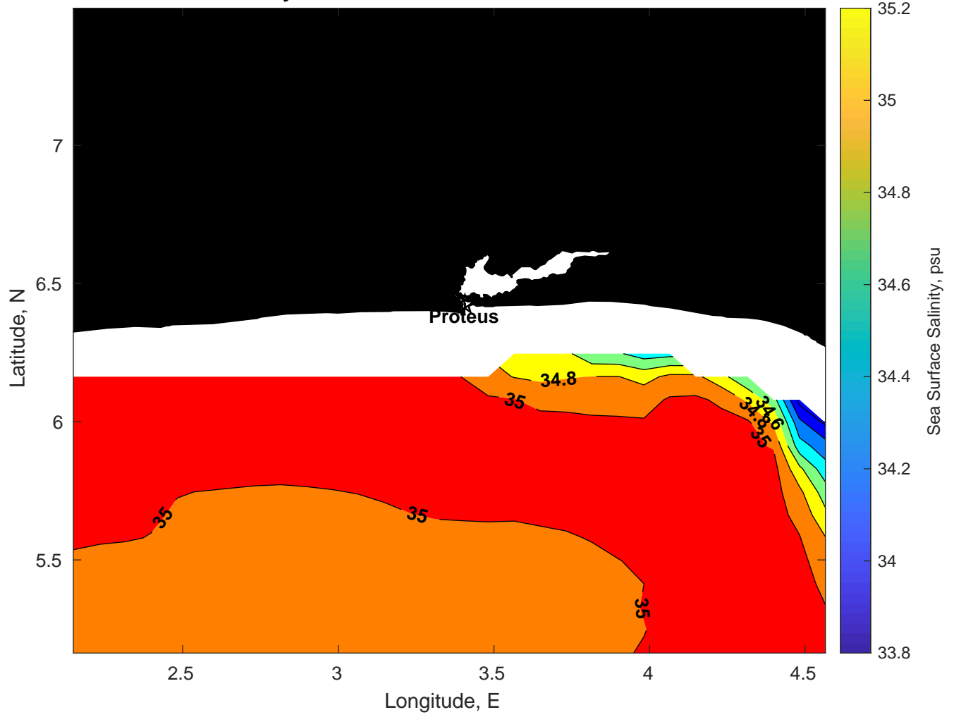
Surface Salinity for Proteus at 02-Mar-2025 00:00:00
