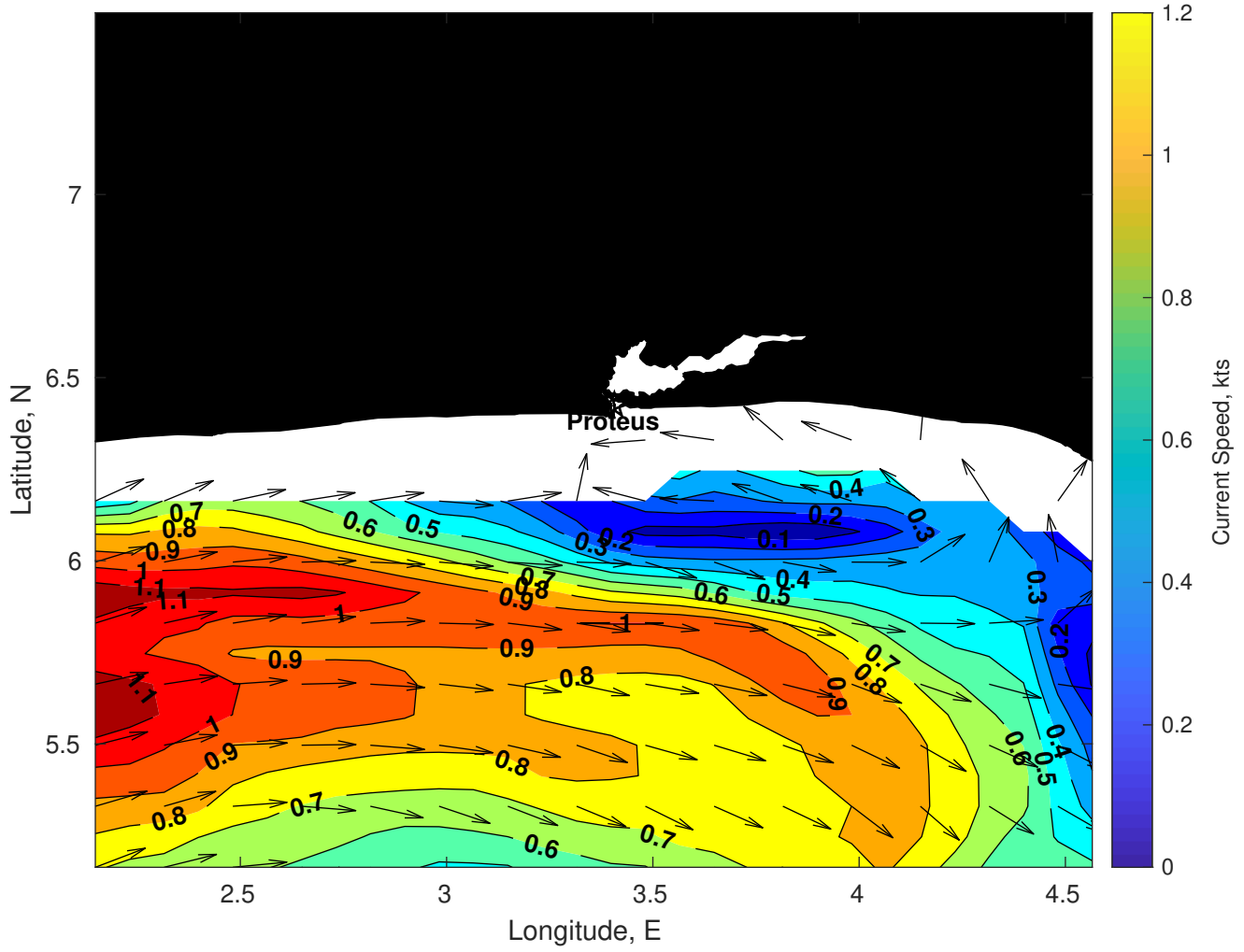
Surface Currents for Proteus at 02-Mar-2025 00:00:00
