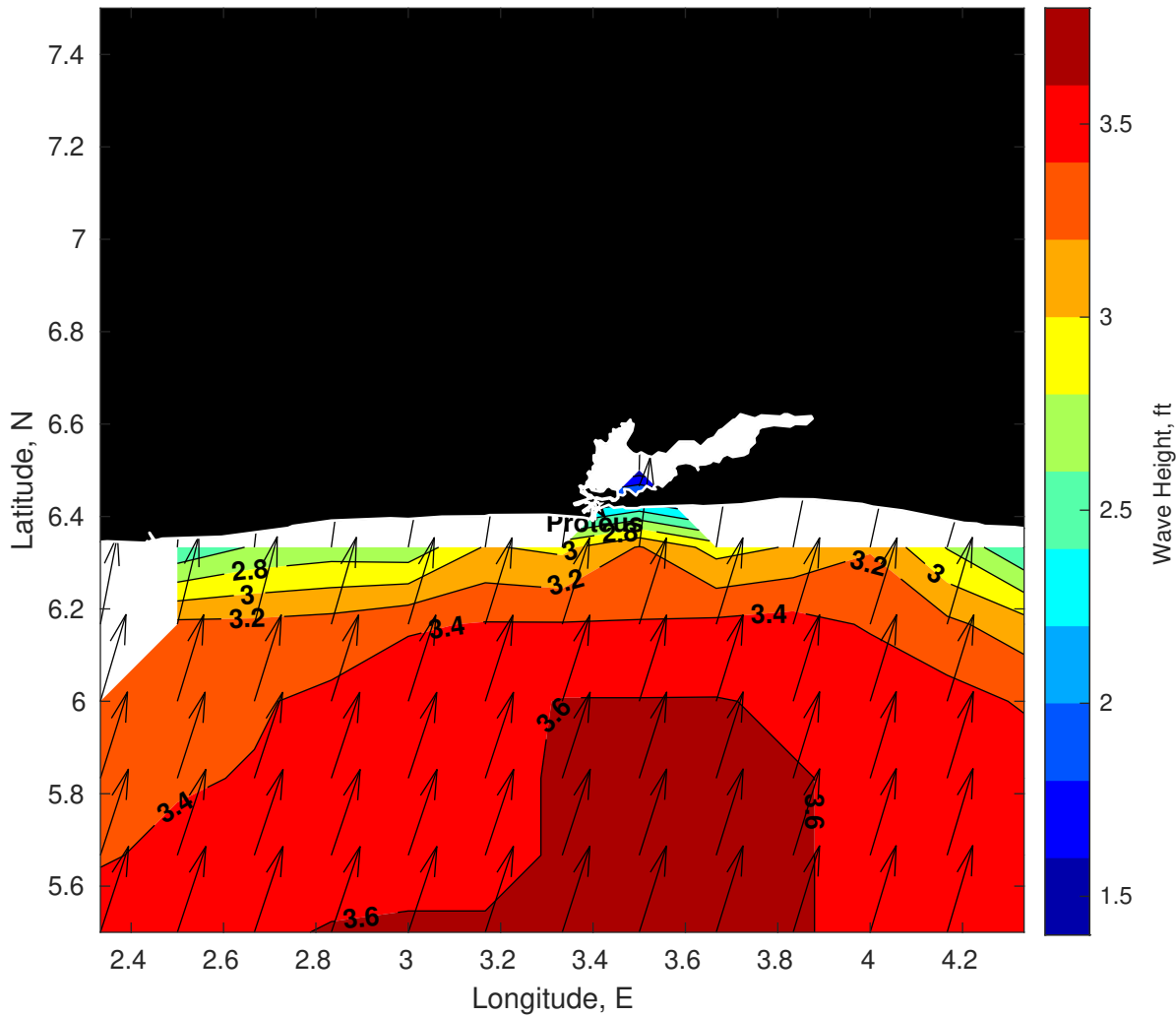
Wave Height (ft) for Proteus at 03-Mar-2025 09:00:00
