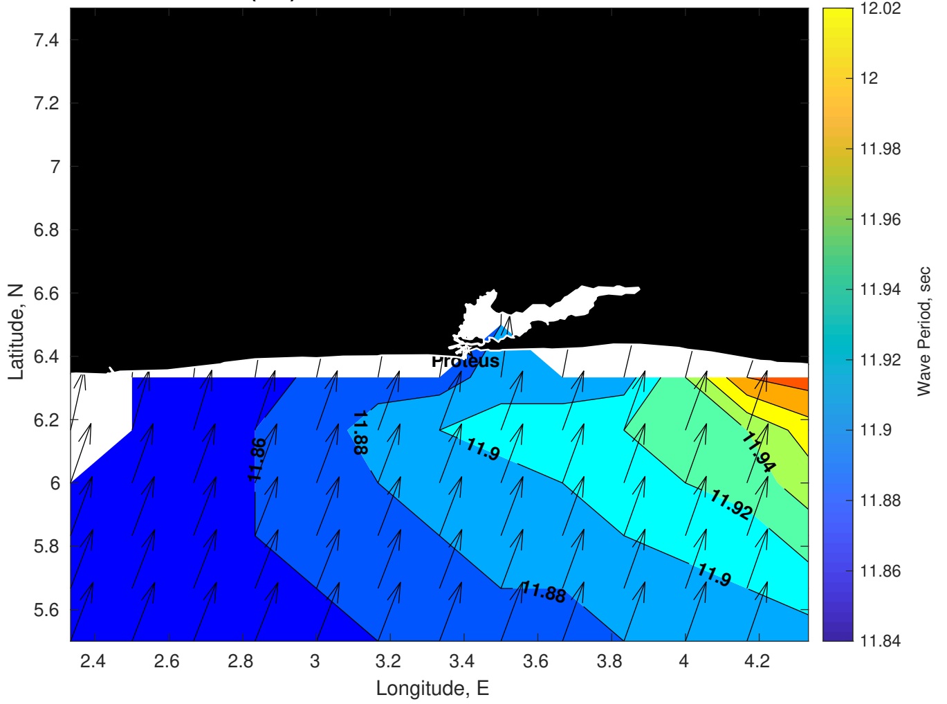
Wave Period (sec) for Proteus at 03-Mar-2025 09:00:00
