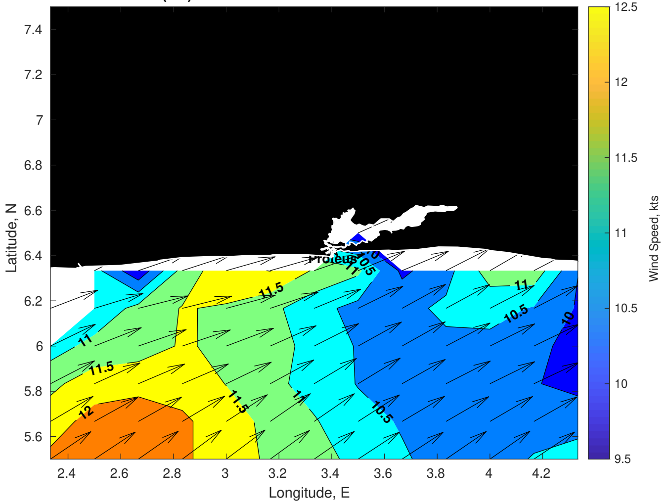
Winds (kts) for Proteus at 03-Mar-2025 09:00:00
