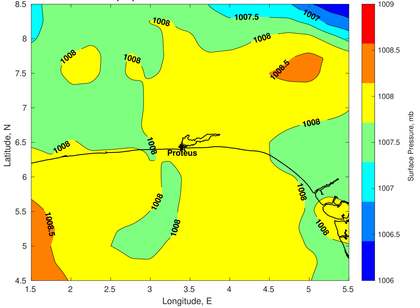
Surface Pressure (mb) for Proteus at 05-Mar-2025 00:00:00
