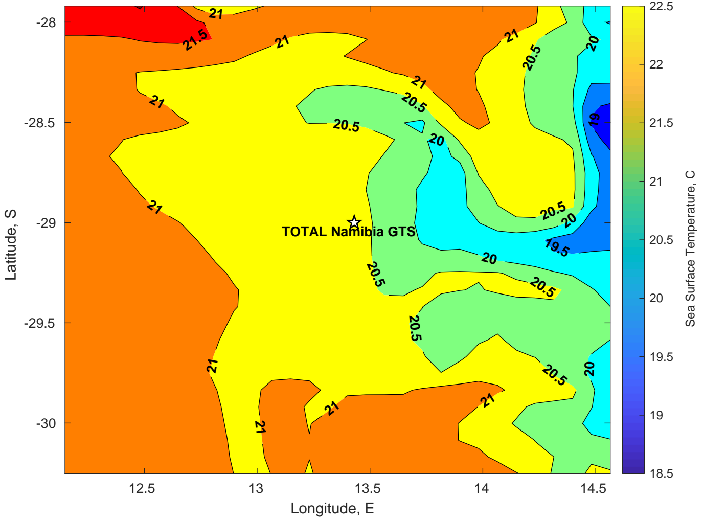
SST for TOTAL Namibia GTS at 02-Mar-2025 00:00:00
