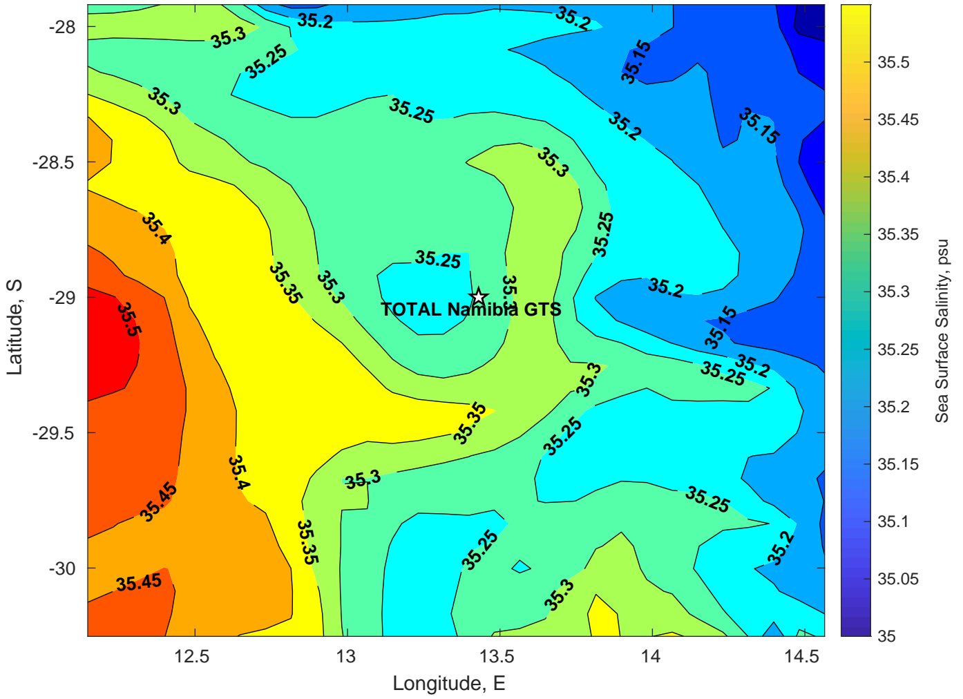
Surface Salinity for TOTAL Namibia GTS at 02-Mar-2025 00:00:00
